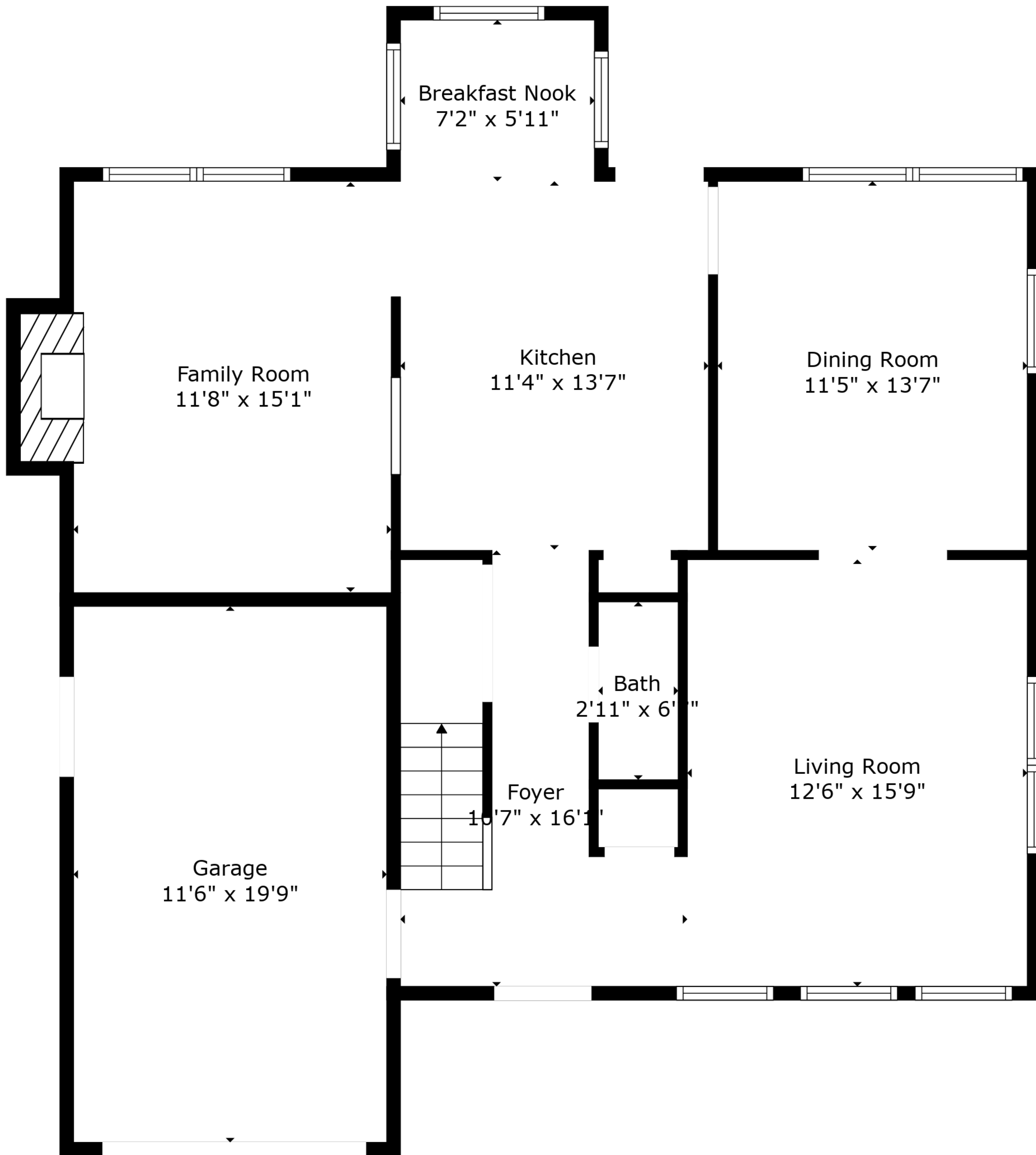
Floor 1
