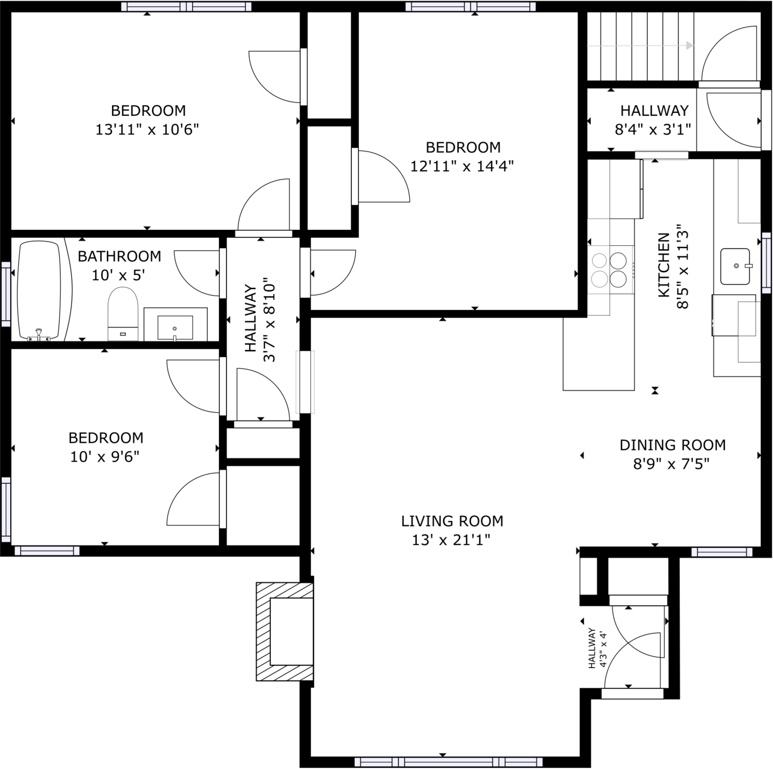
FLOOR 2
