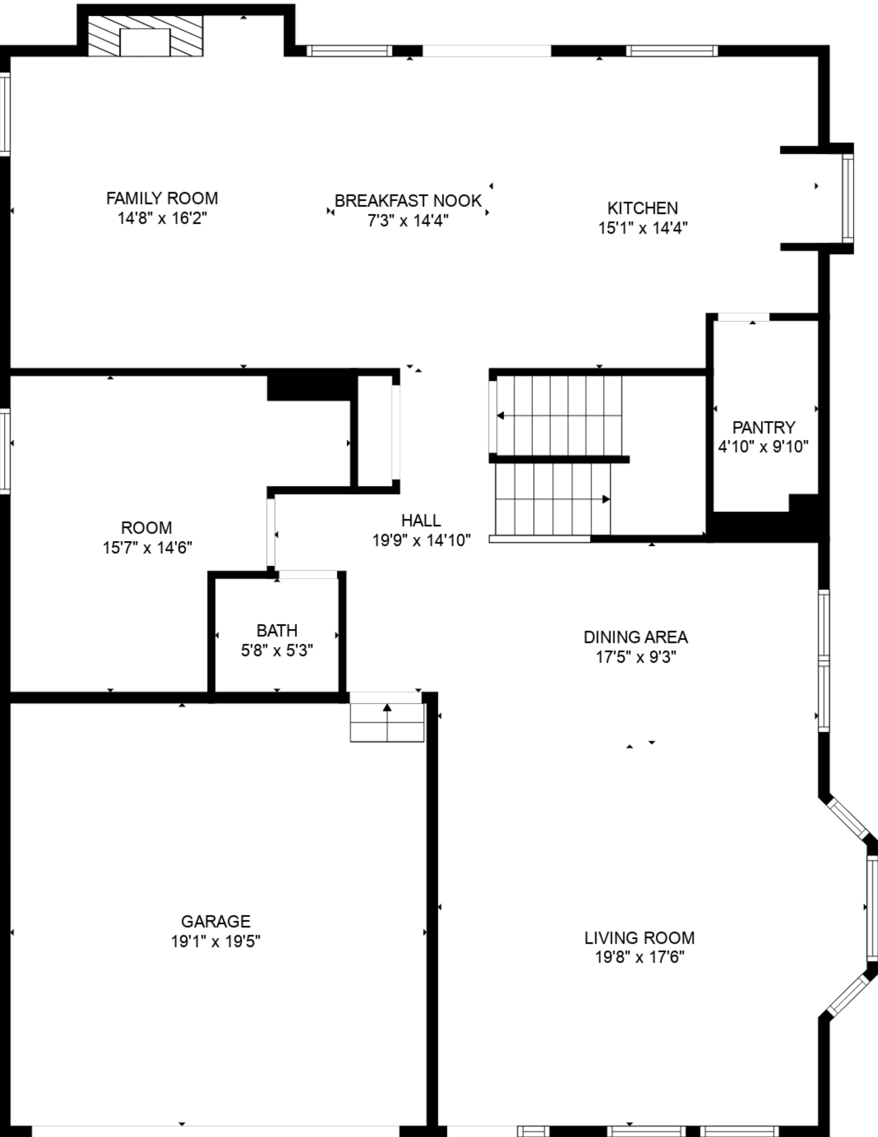
FLOOR 2
