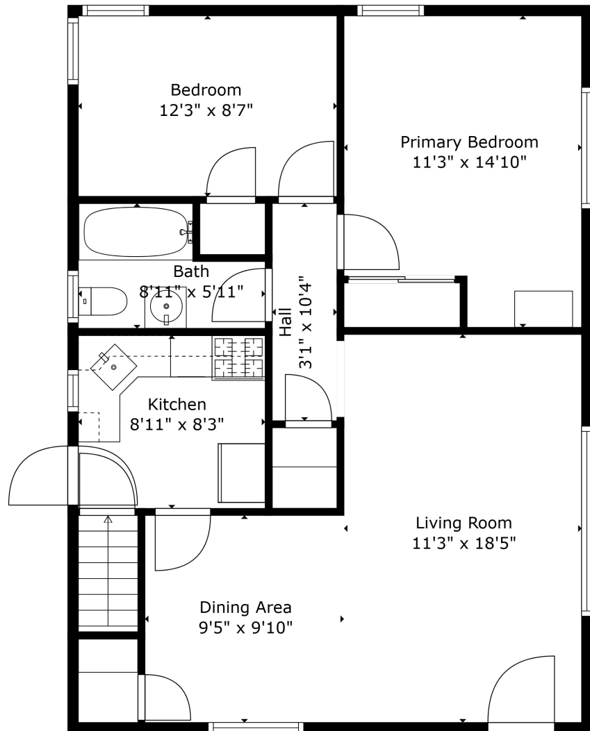
Floor 2
