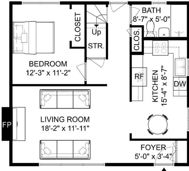
MAIN FLOOR 719 sq.ft. | Ceiling Height: 8'-0"
