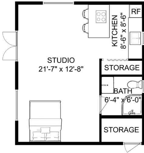
MAIN FLOOR 719 sq.ft. | Ceiling Height: 8'-0"
