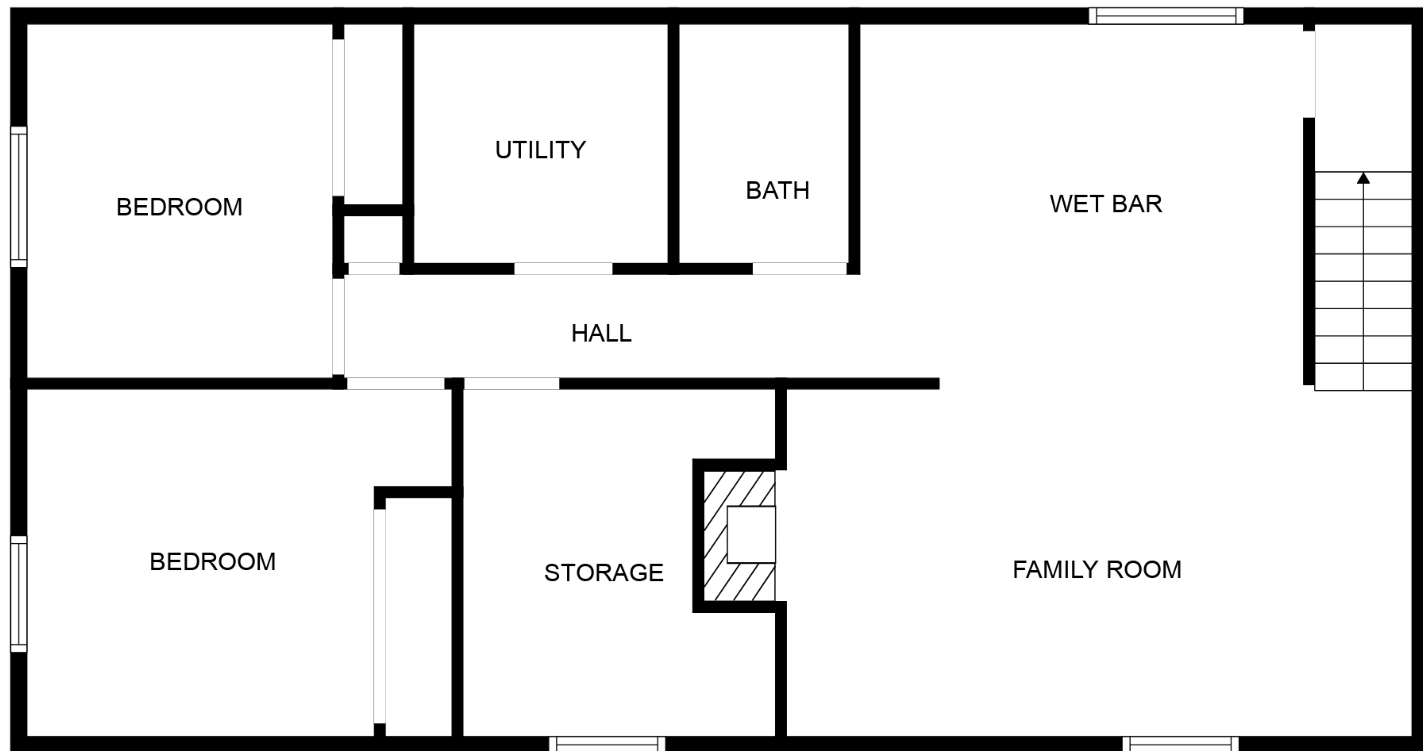
FLOOR 1
