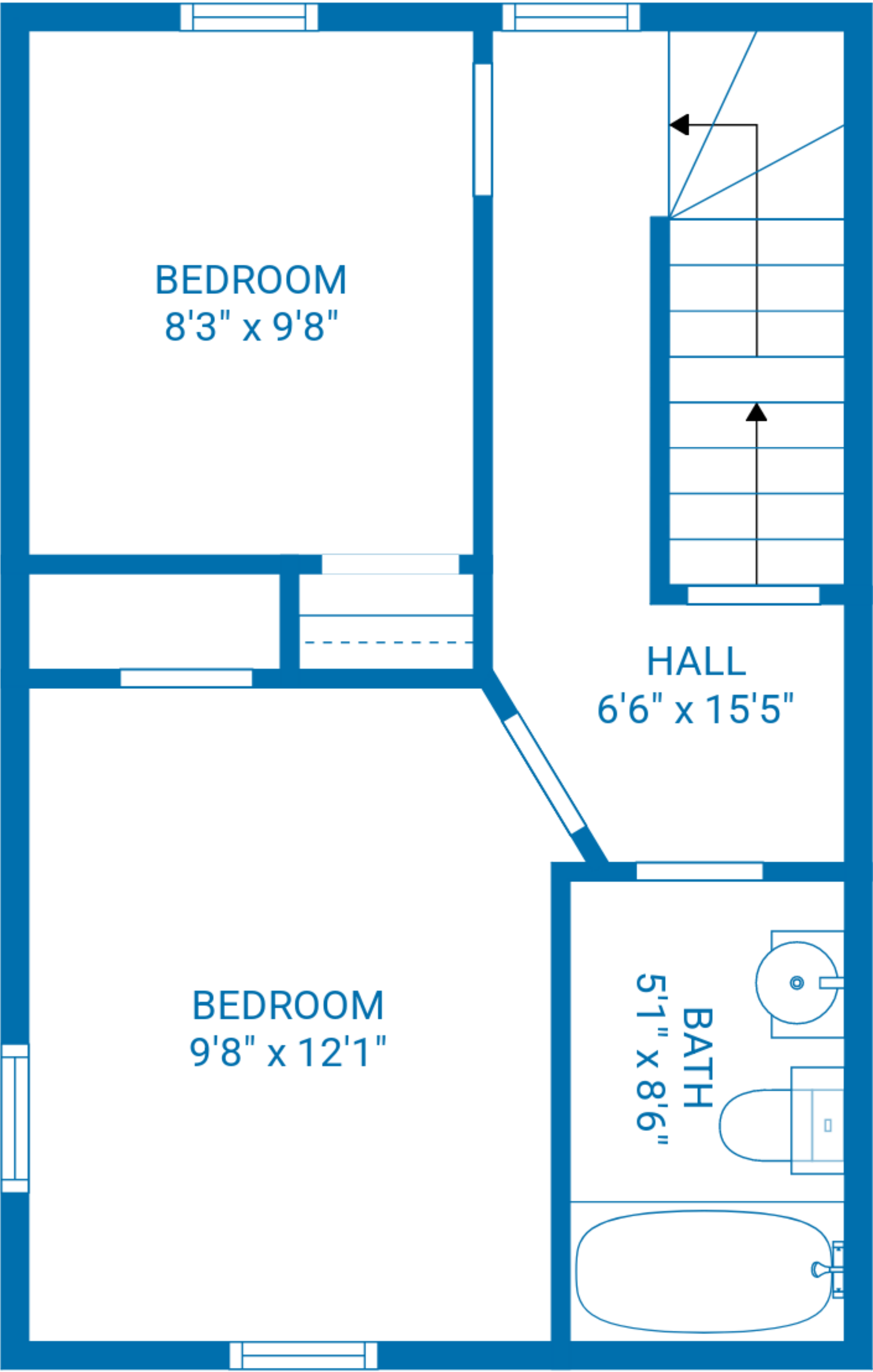
FLOOR 3
