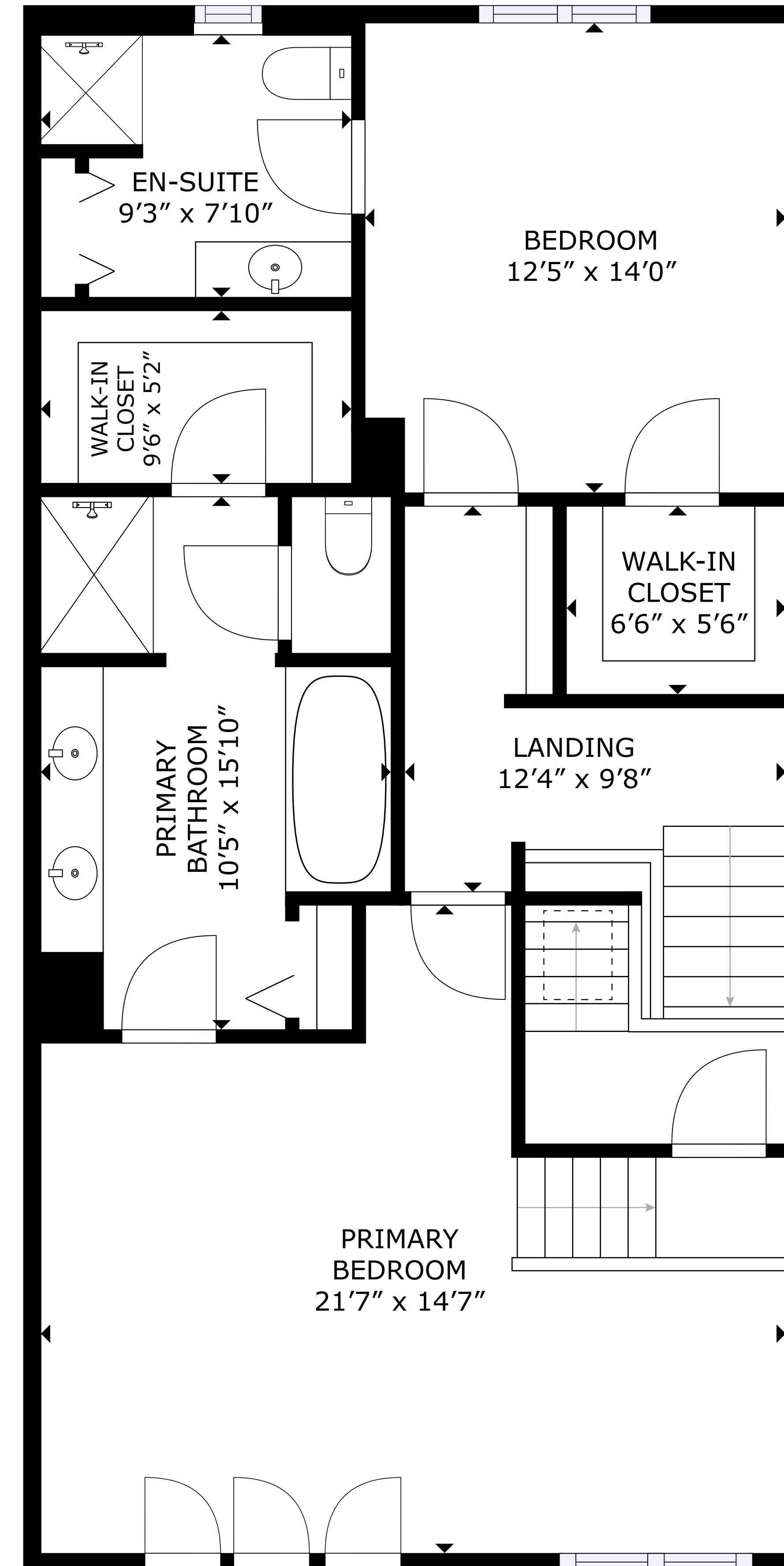
2ND FLOOR
