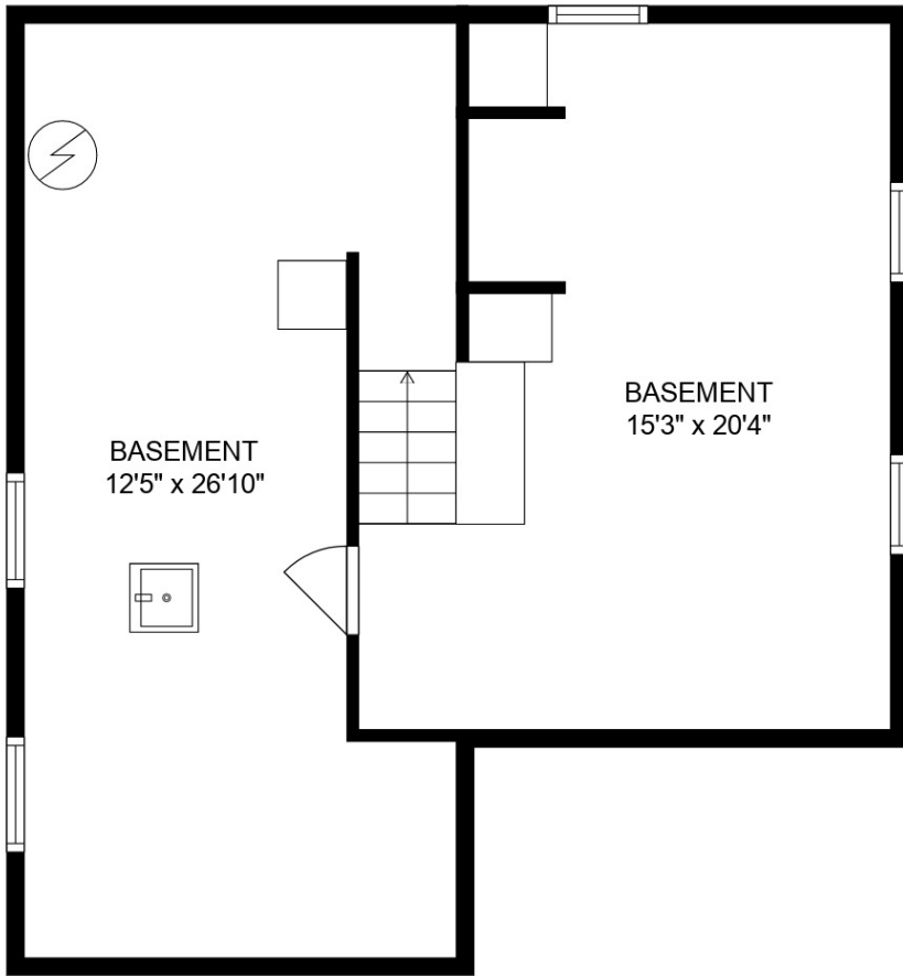
LOWER FLOOR
