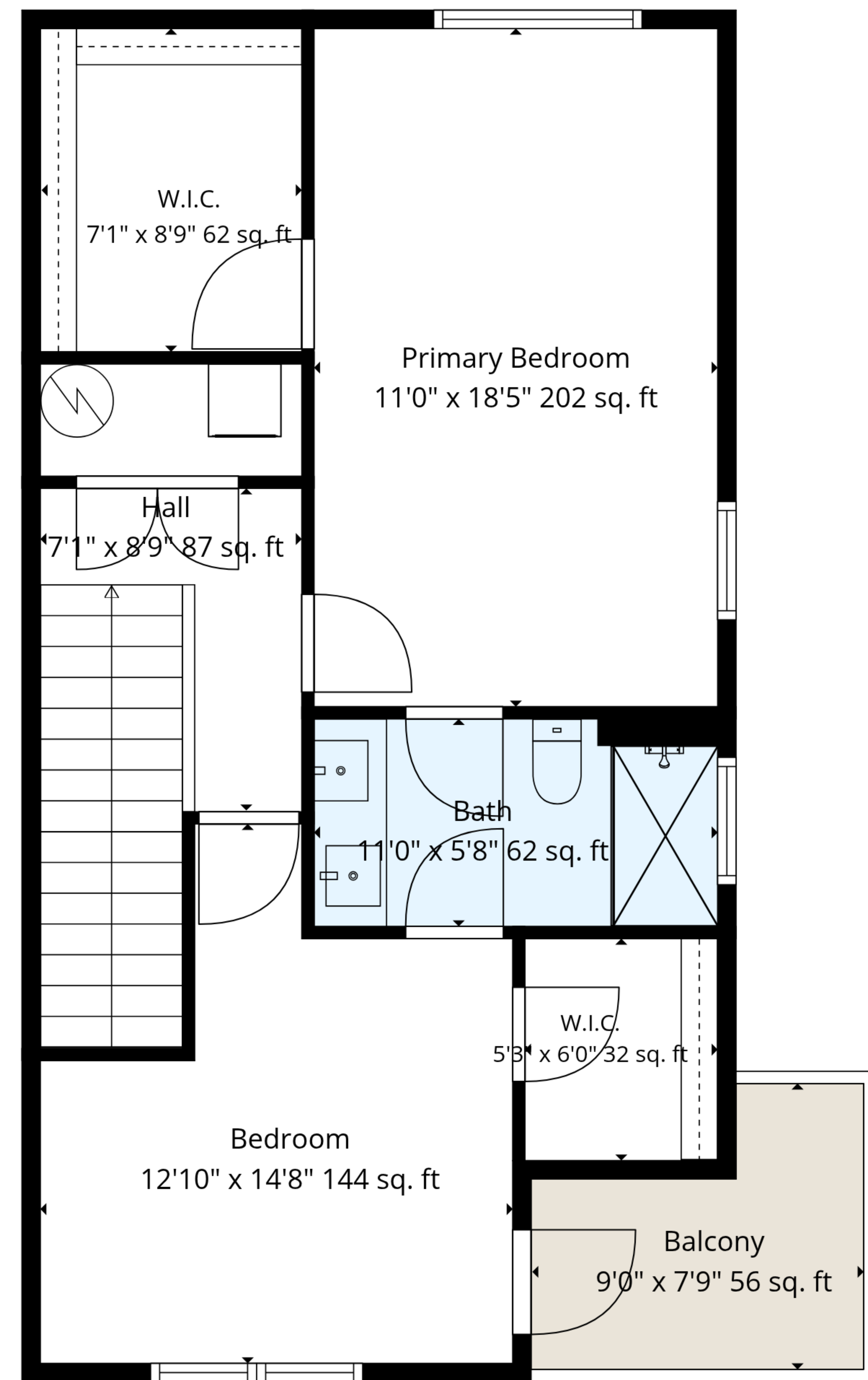
2nd Floor
