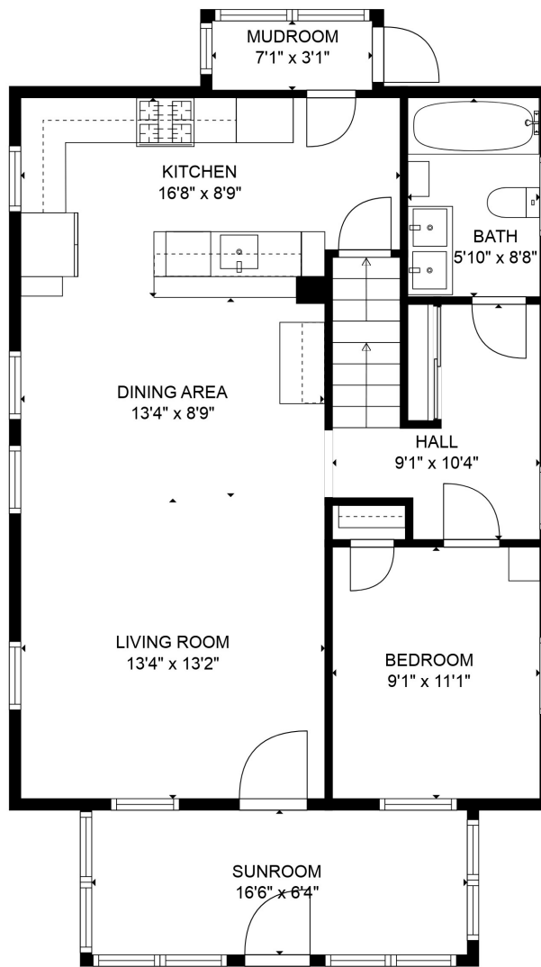
FLOOR 2
