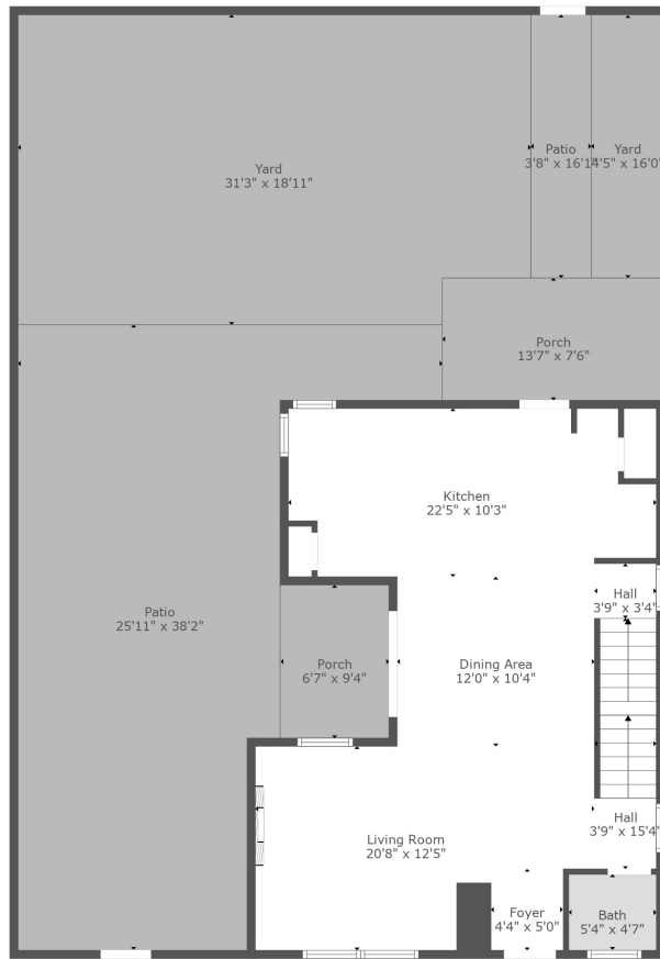
Floor 2
