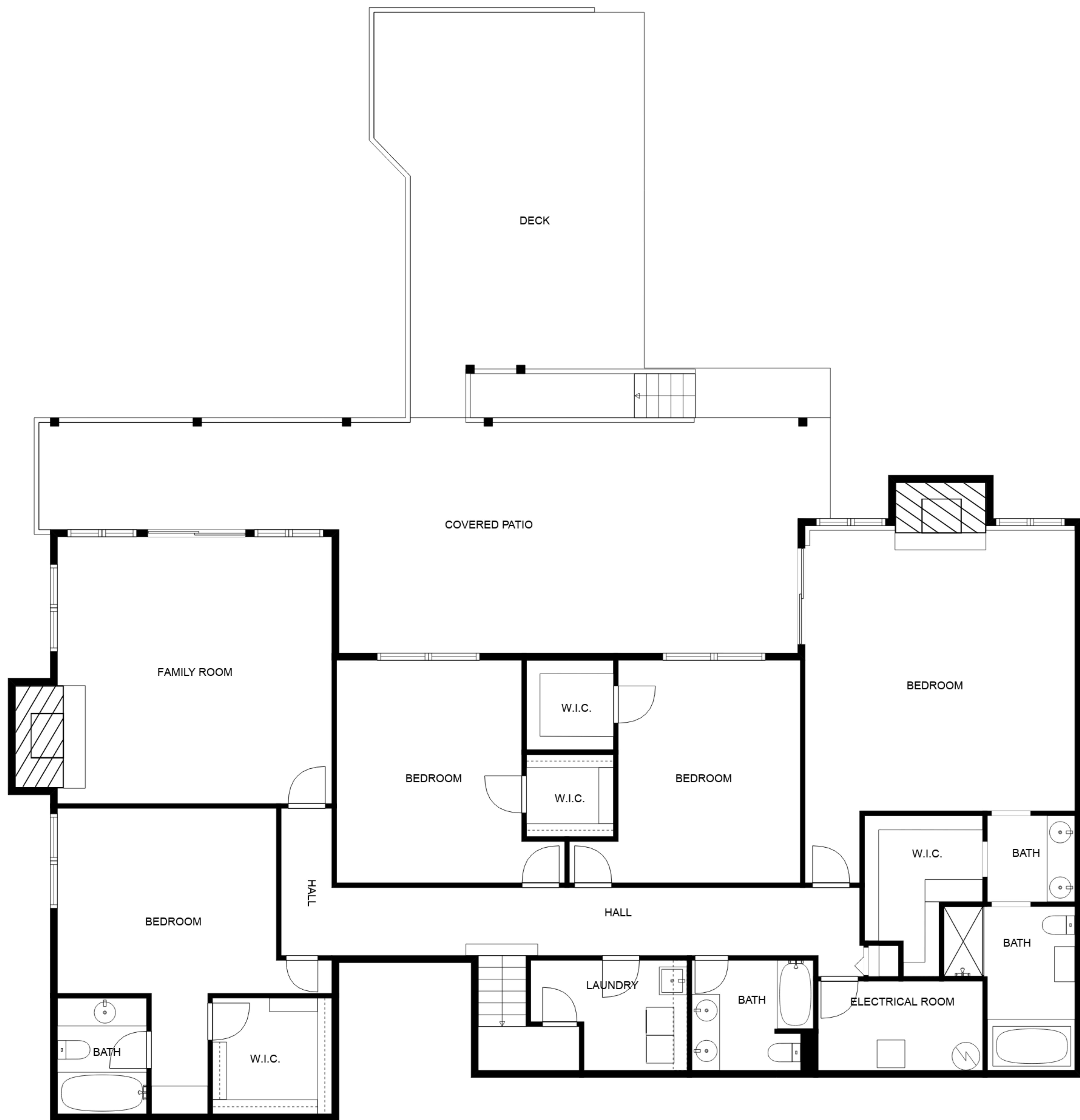
FLOOR 1
