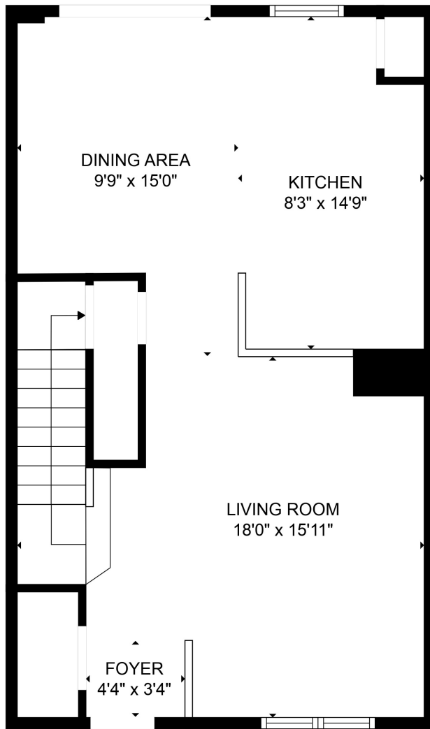
FLOOR 1
