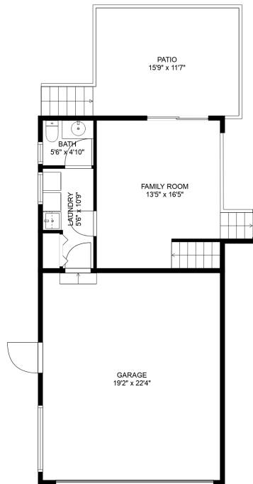
FLOOR 2
