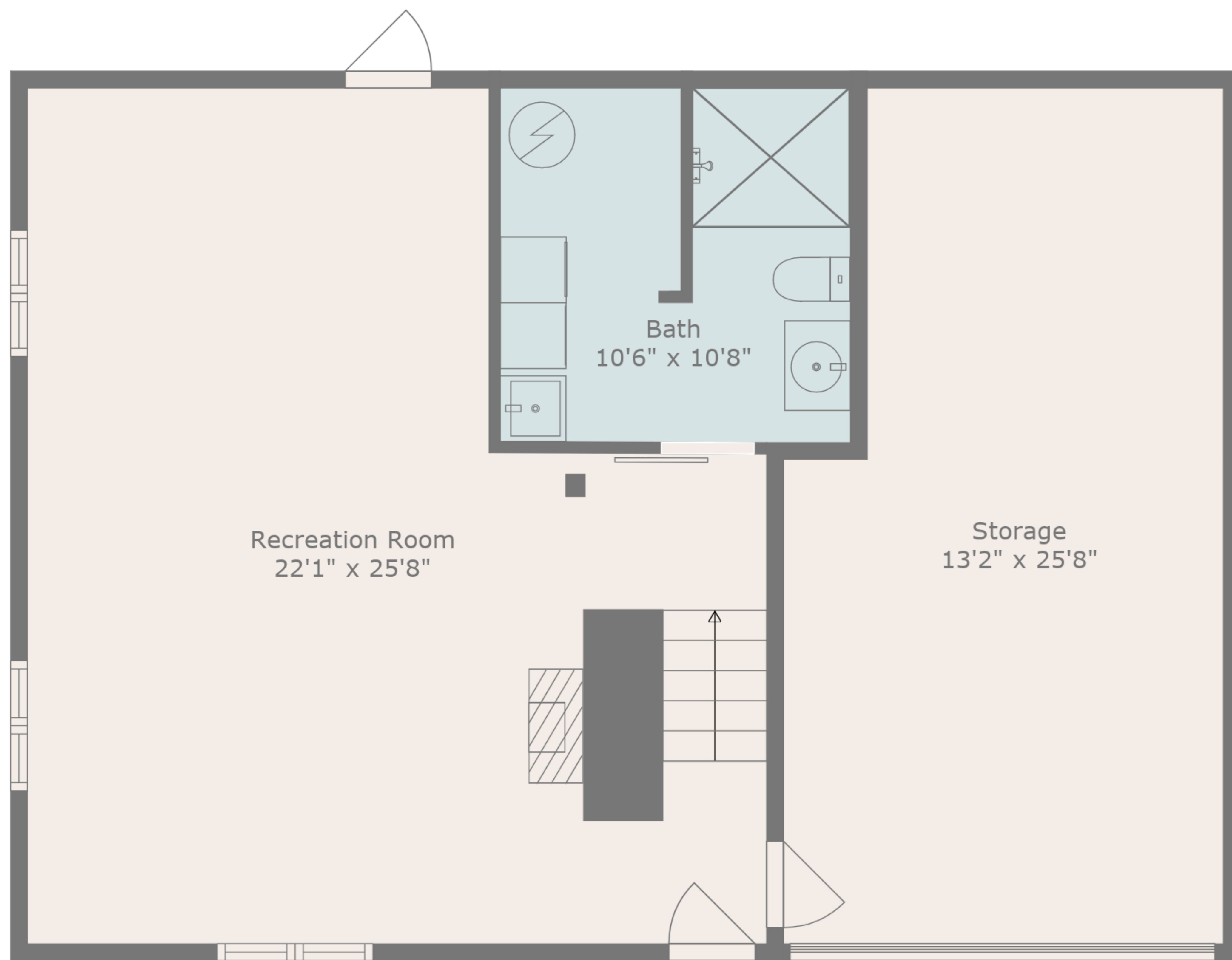
Floor 1
