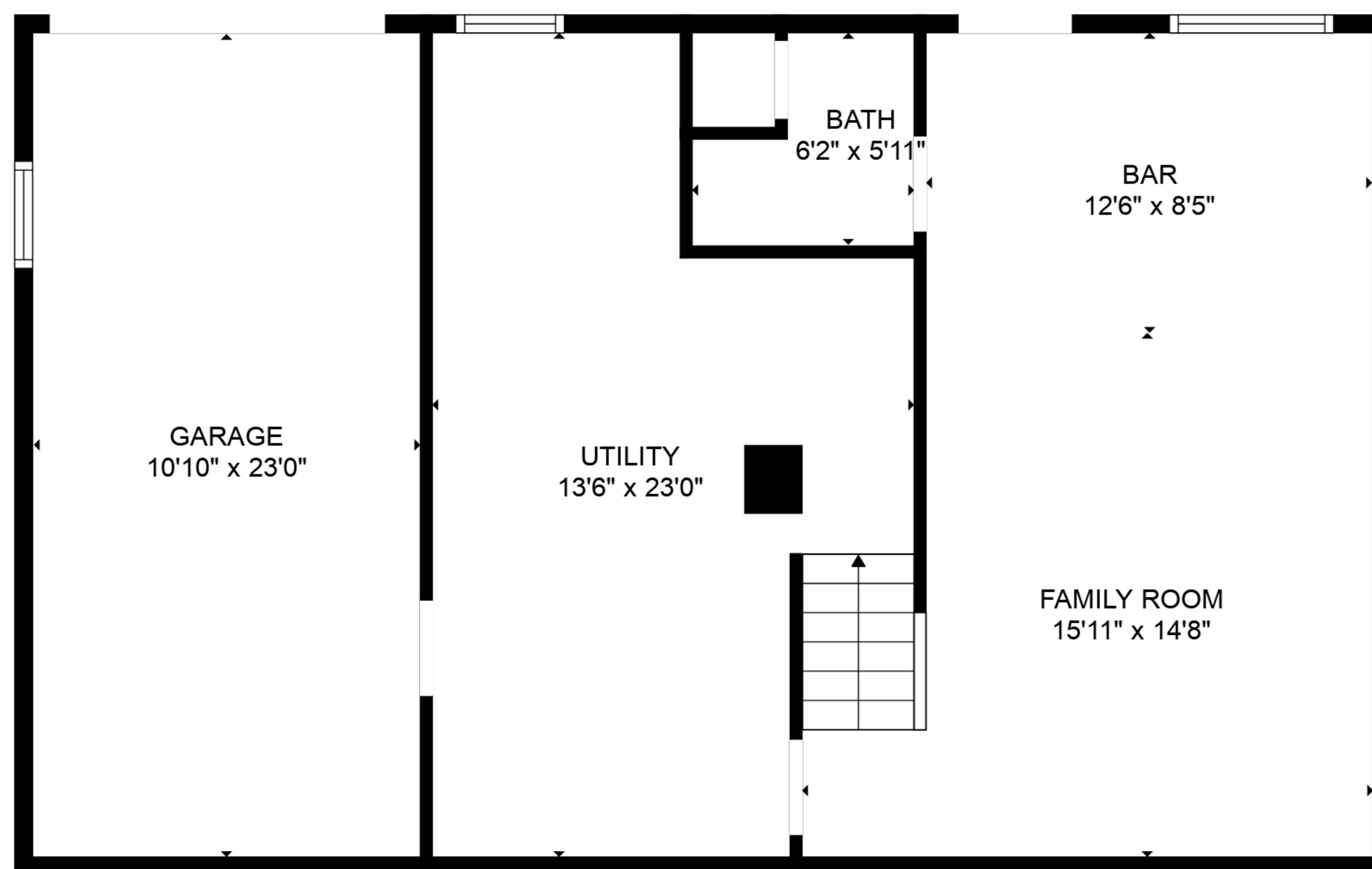
FLOOR 1
