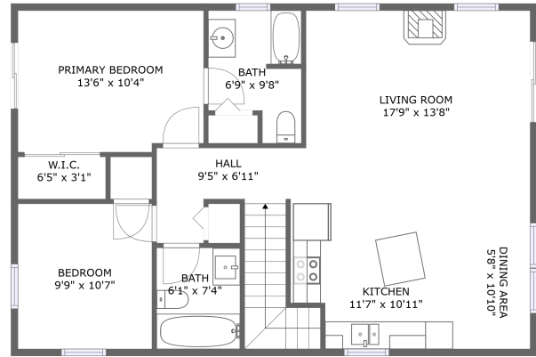
FLOOR 2
