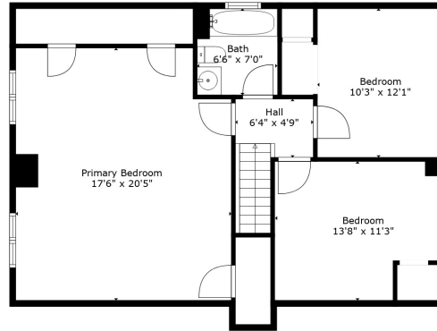
Floor 3
