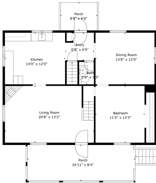
Floor 2
