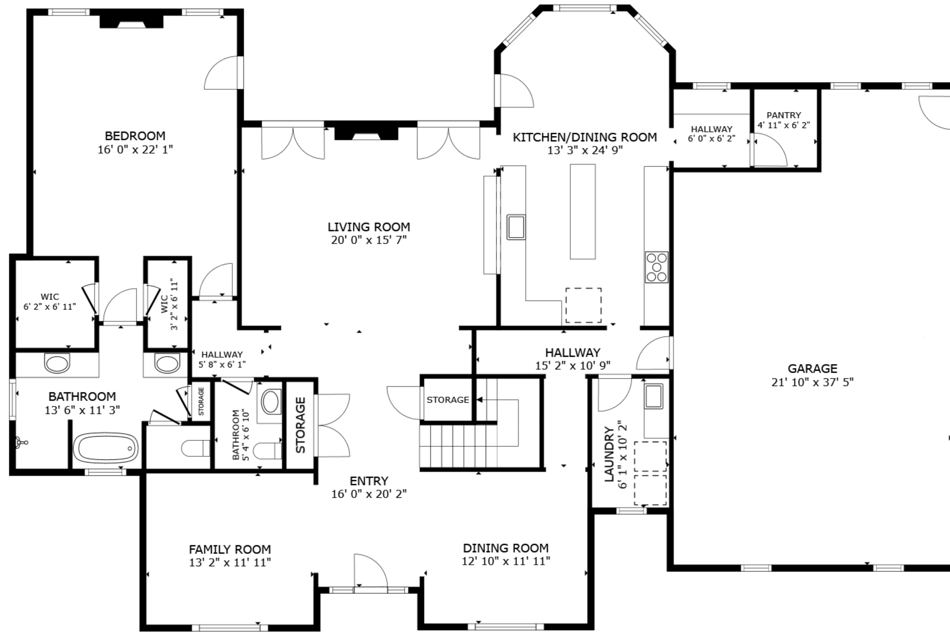
FLOOR 1
