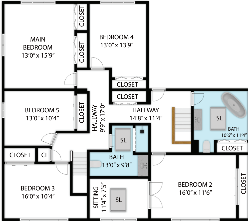
SECOND FLOOR
