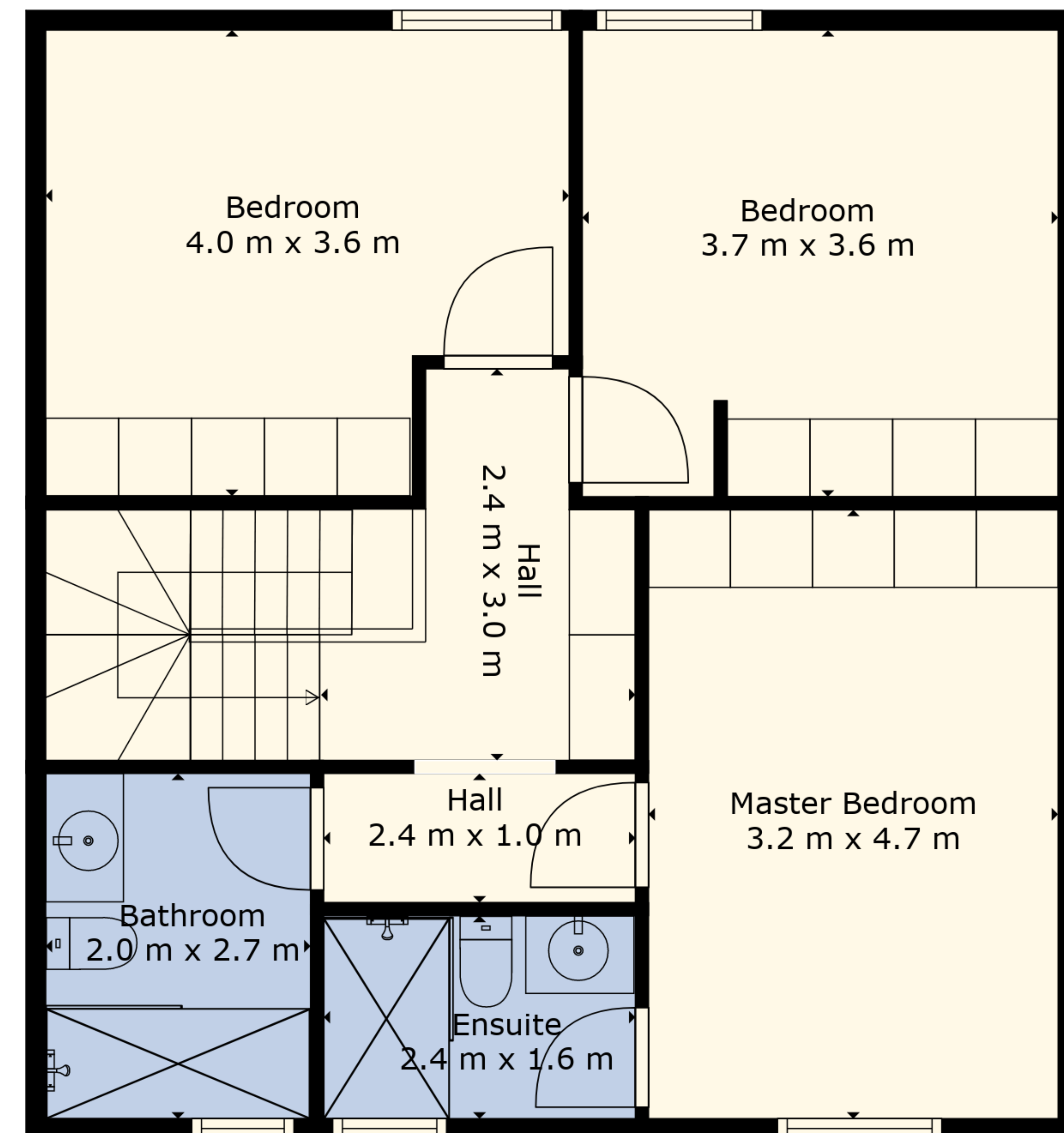
Floor 2
