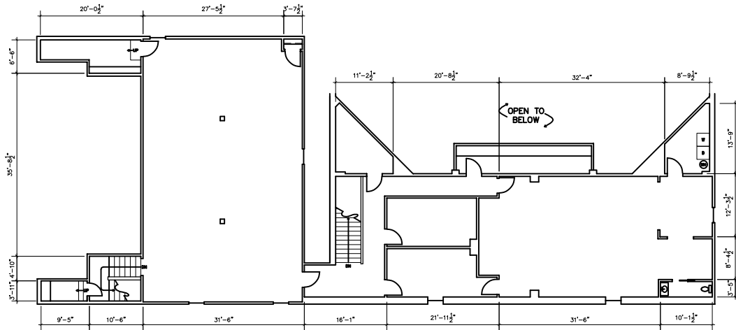
○ SECOND FLOOR
