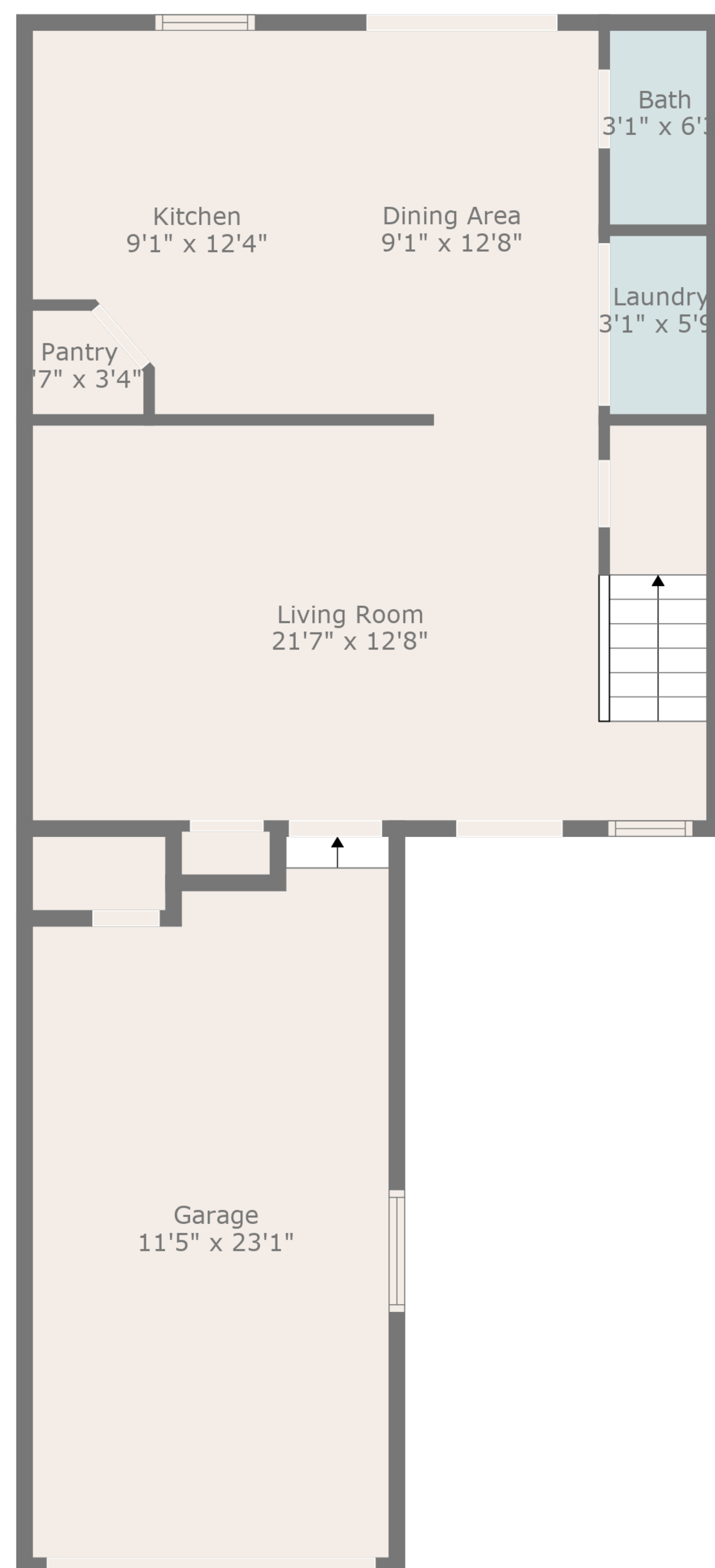
Floor 1
