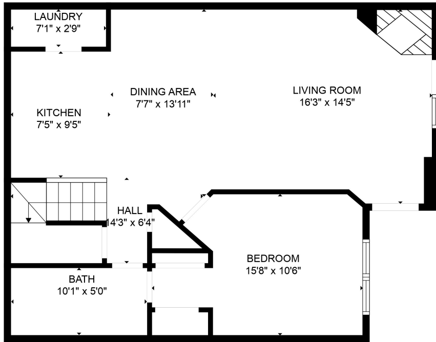
FLOOR 1
