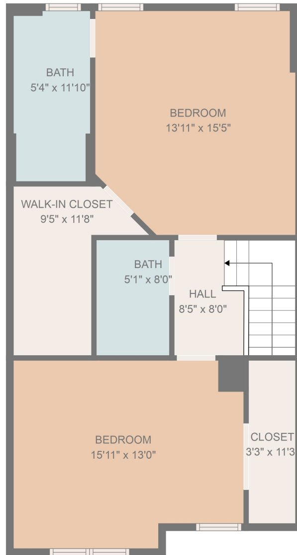
FLOOR 2
