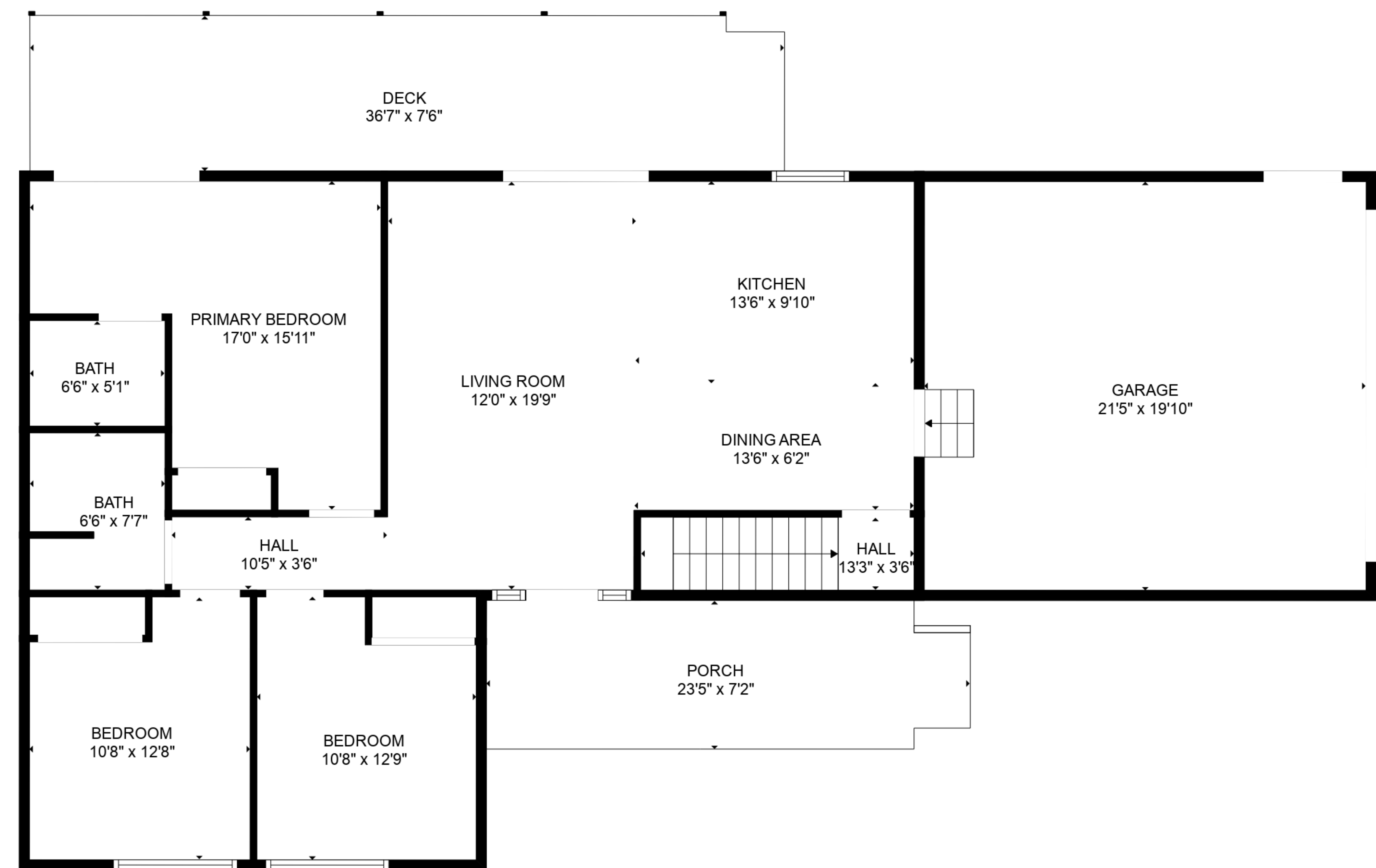
FLOOR 2
