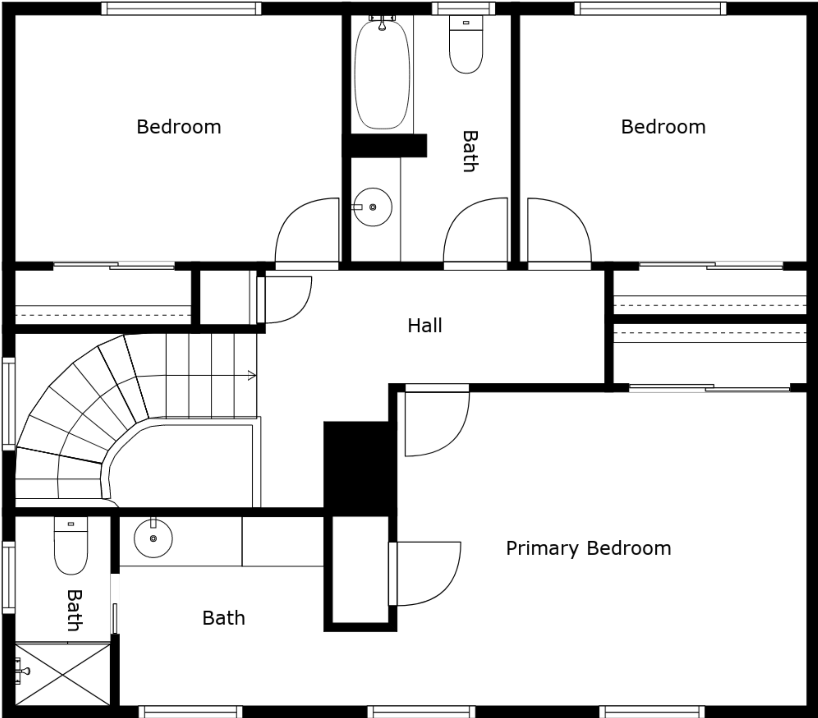
Floor 2
