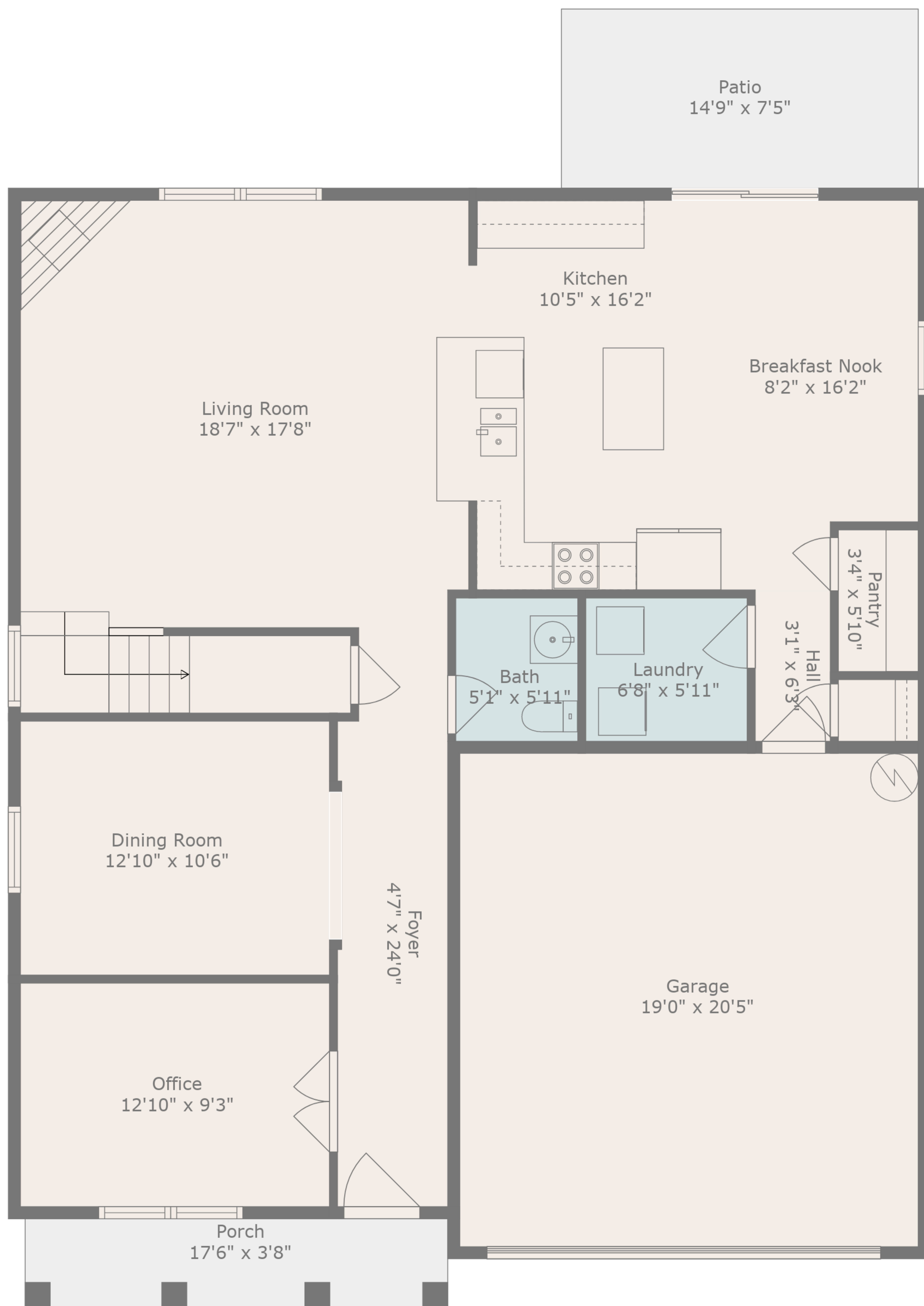
Floor 1
