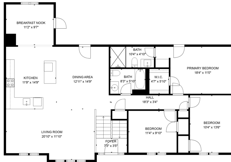
FLOOR 2
