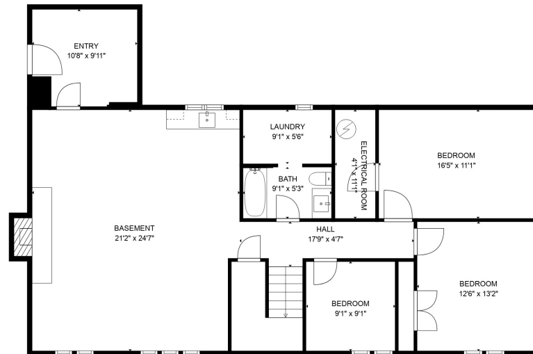
FLOOR 1
