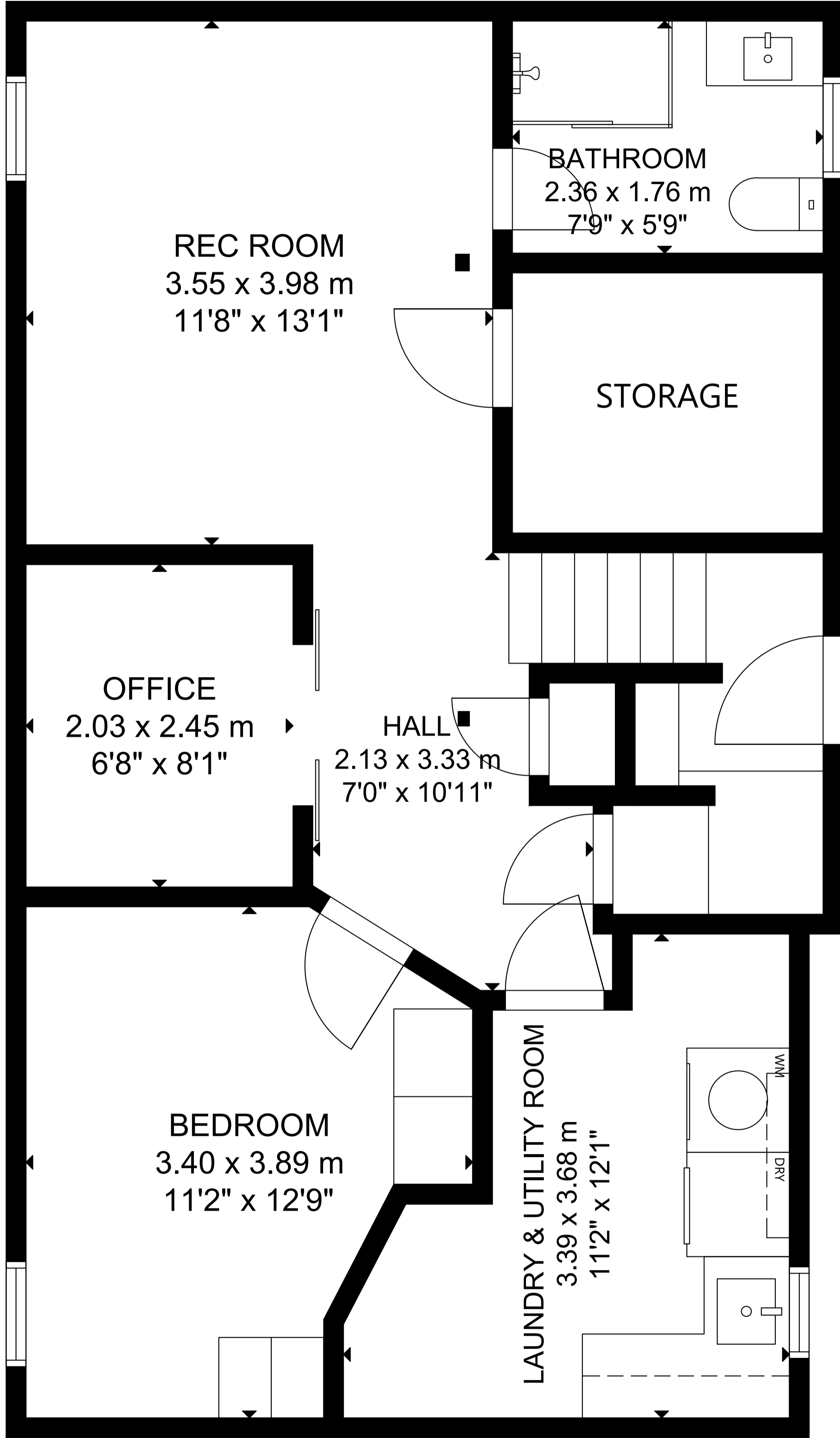
LOWER LEVEL
