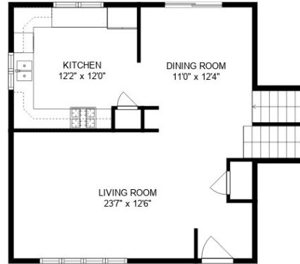
UPPER FLOOR
