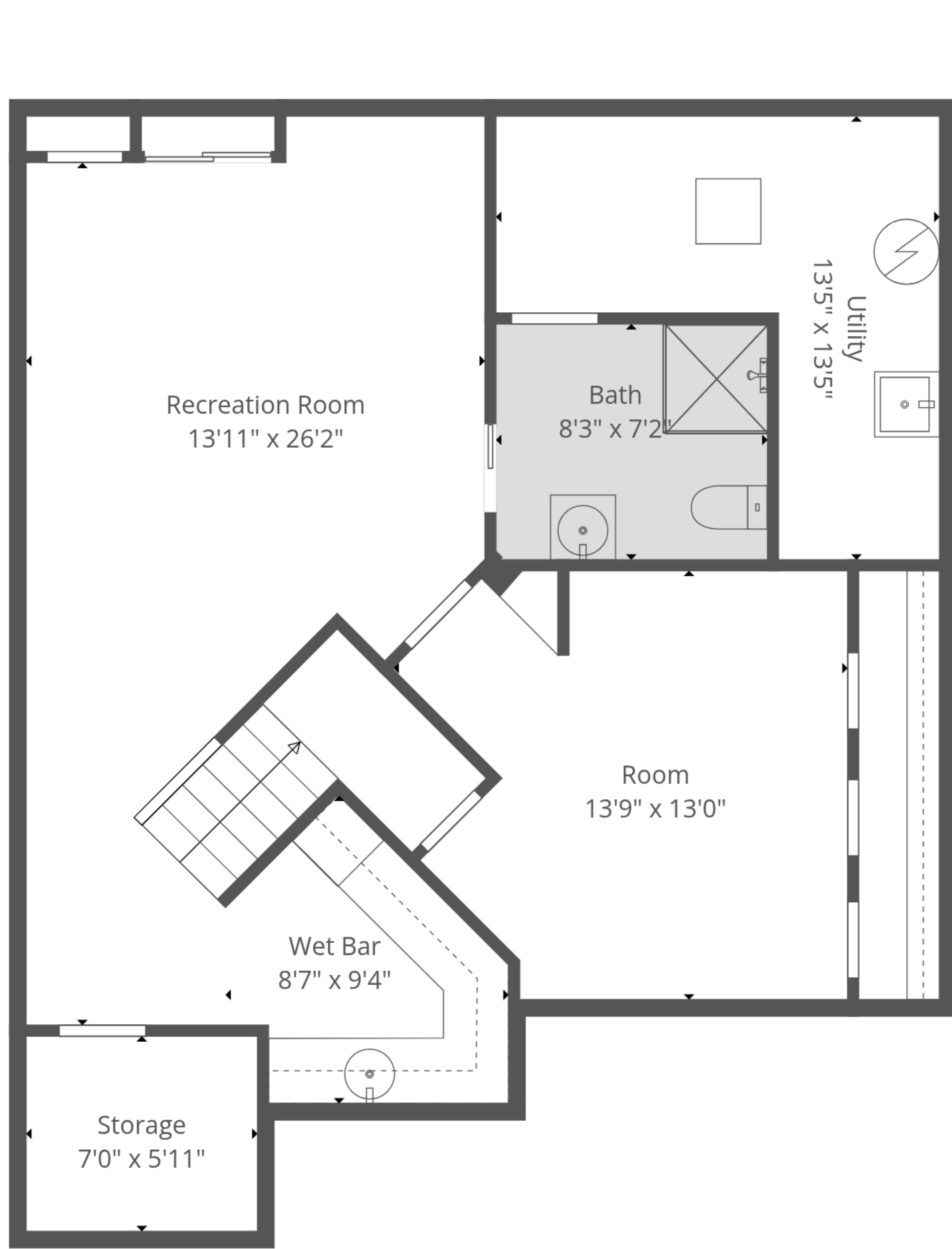
Floor 1
