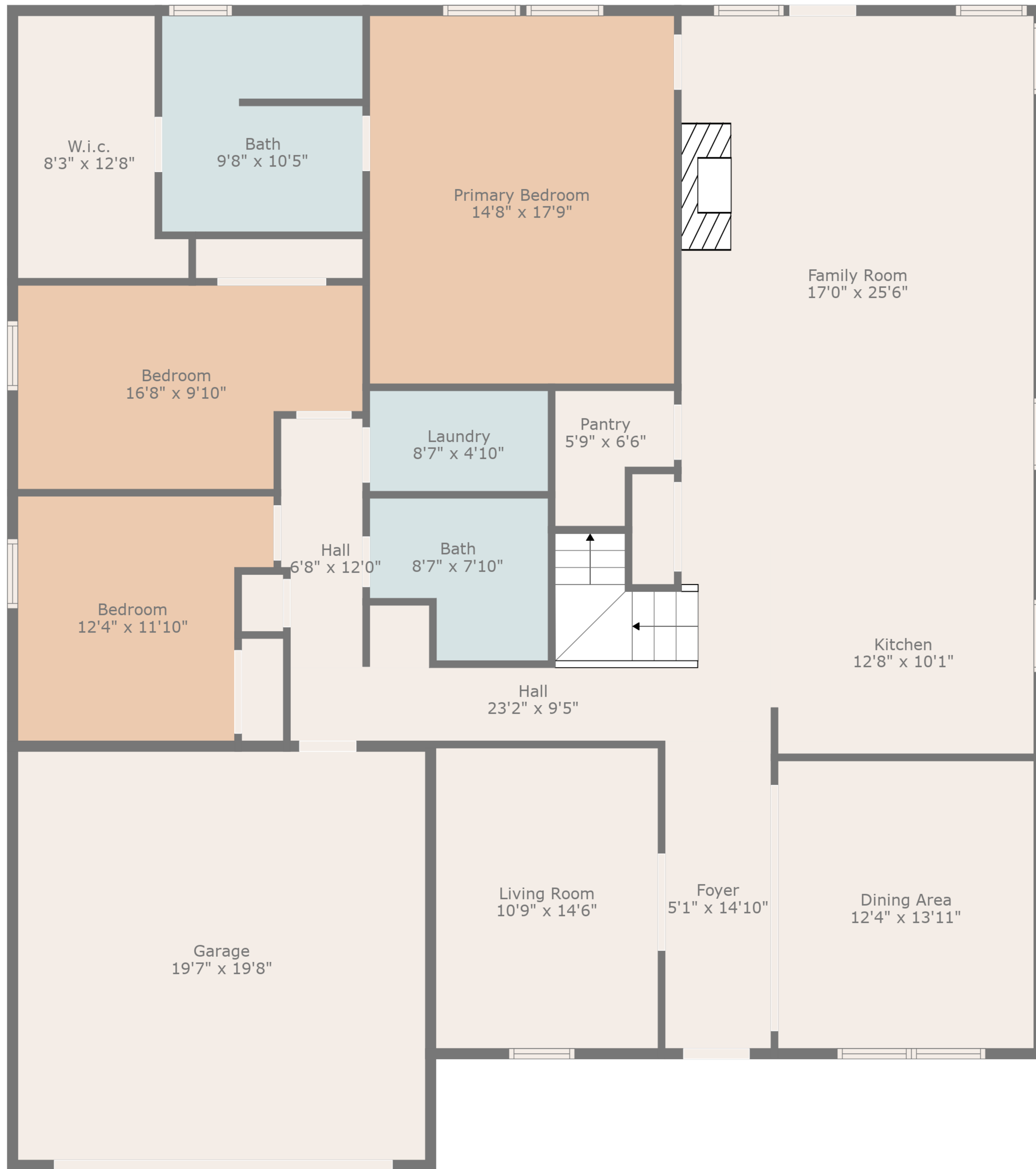
Floor 1
