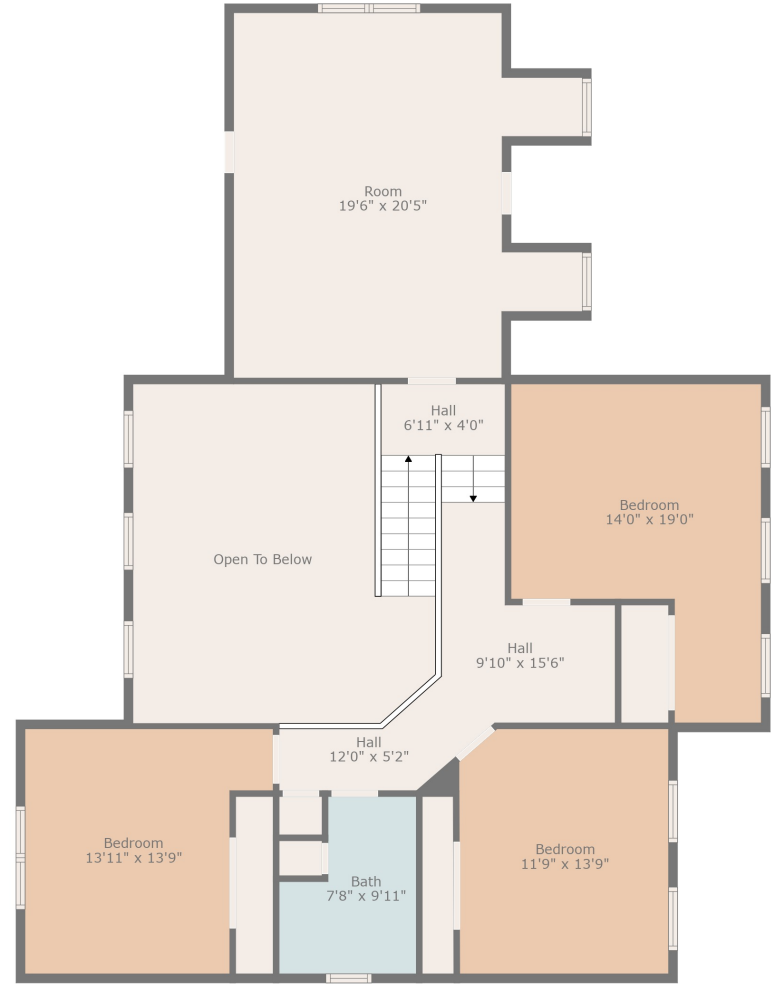
Floor 2
