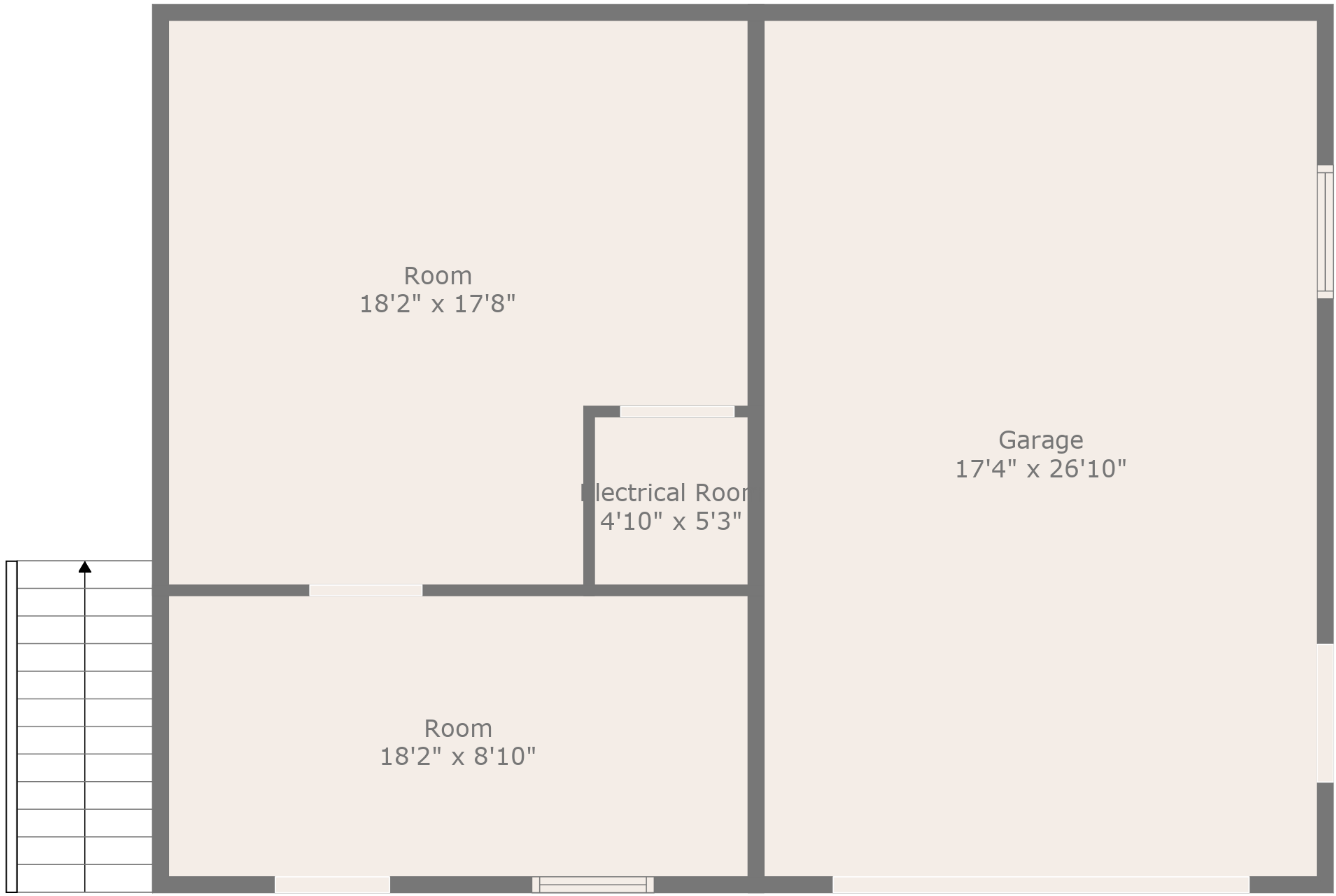
Floor 1
