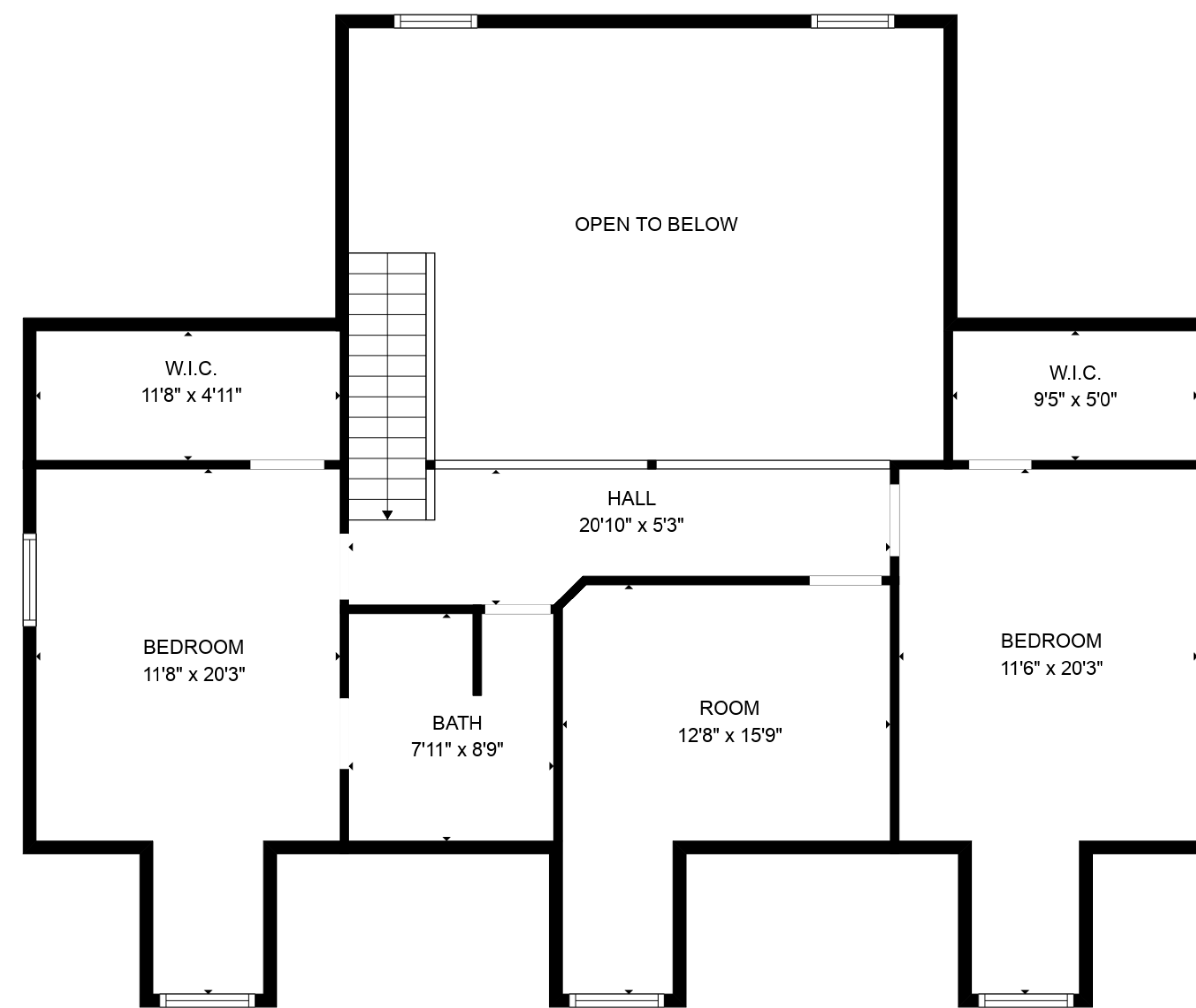
FLOOR 2
