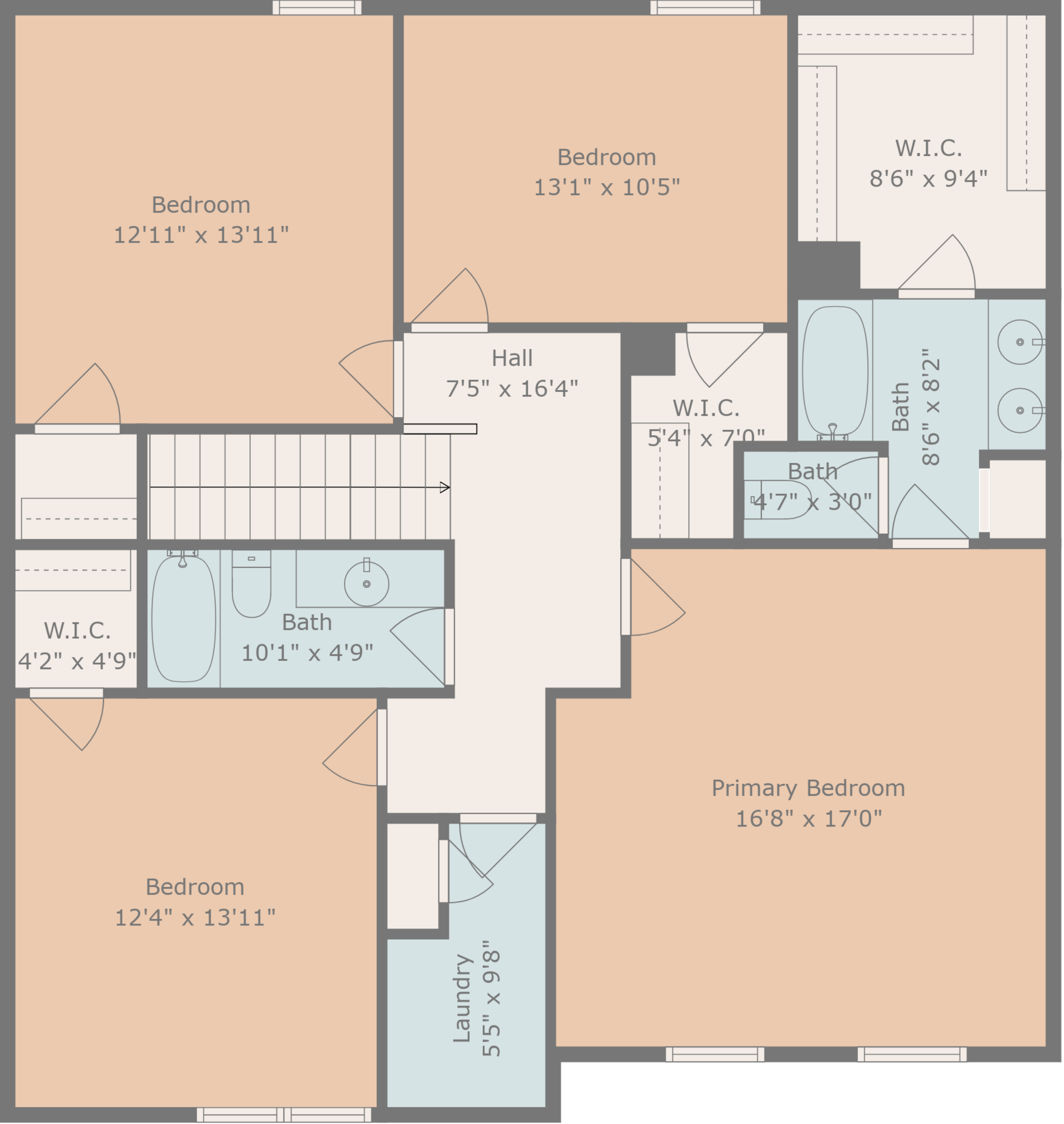
Floor 2
