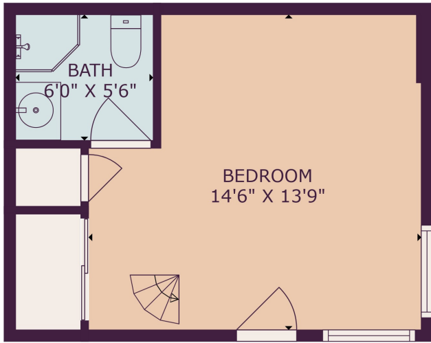
FLOOR 1
