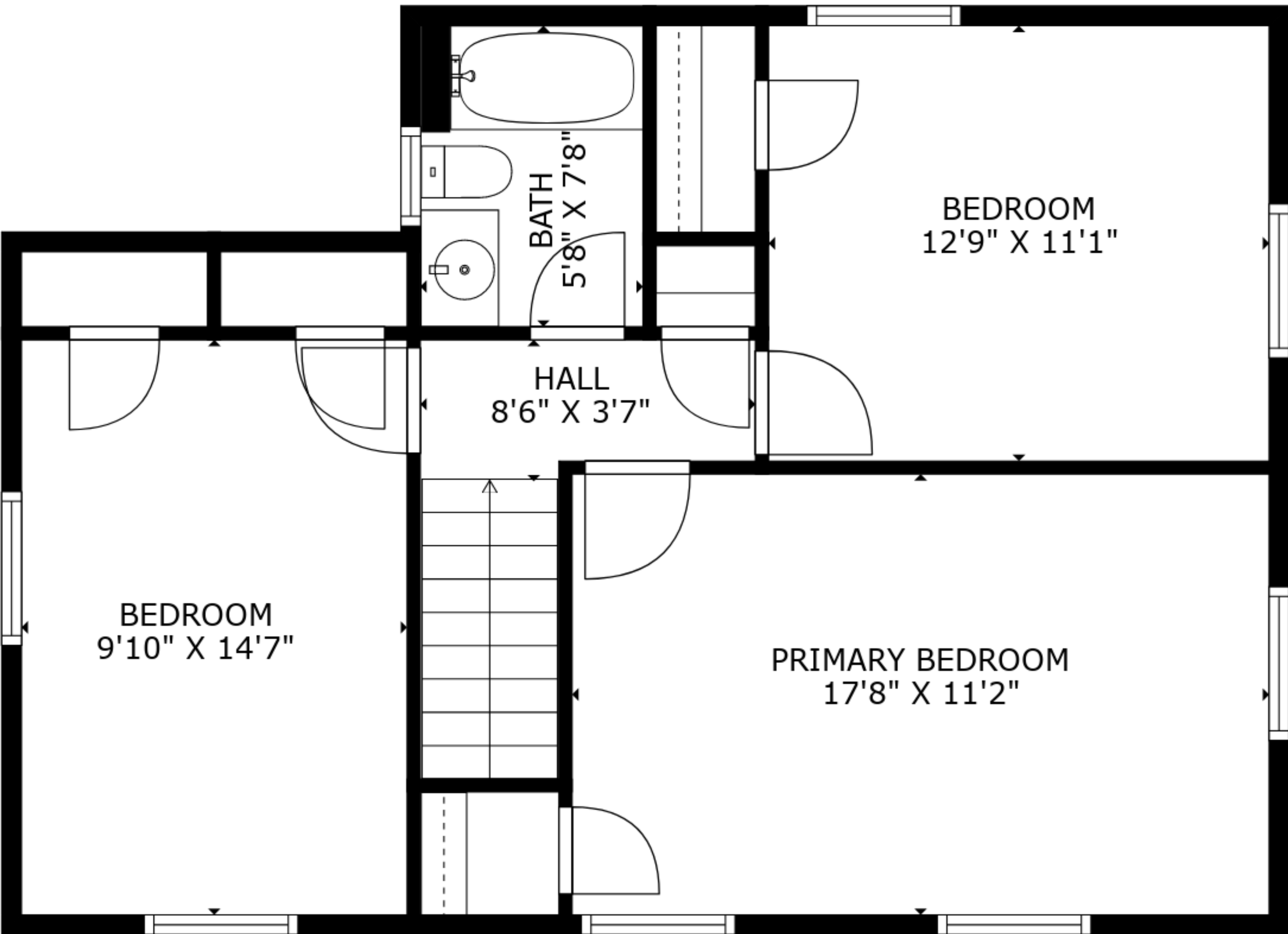
SECOND FLOOR
