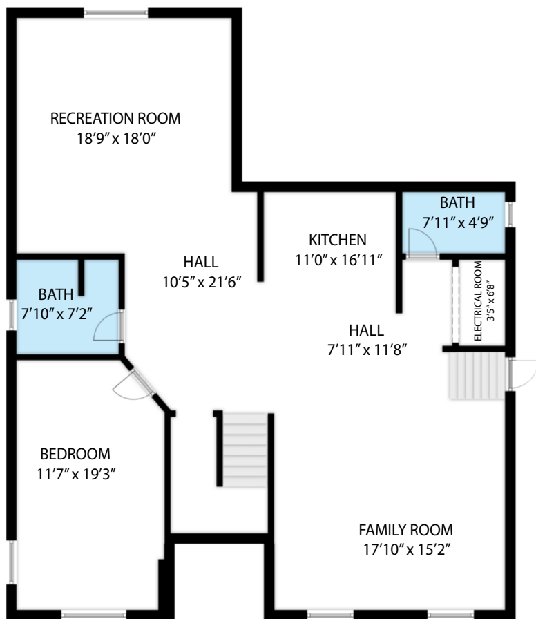
LOWER LEVEL 1,465 SQ.FT
