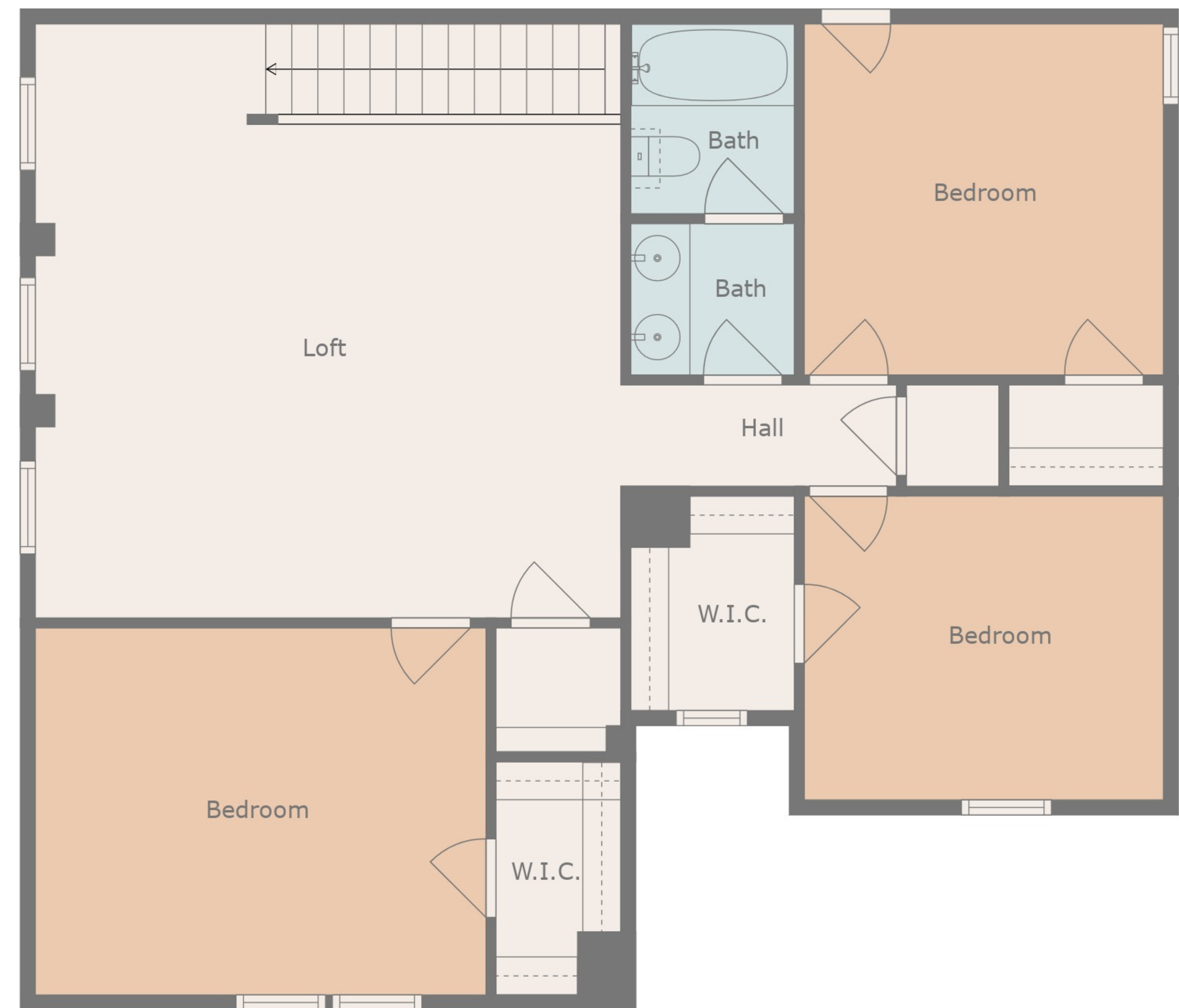
Floor 2
