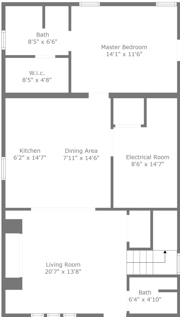
Floor 1
