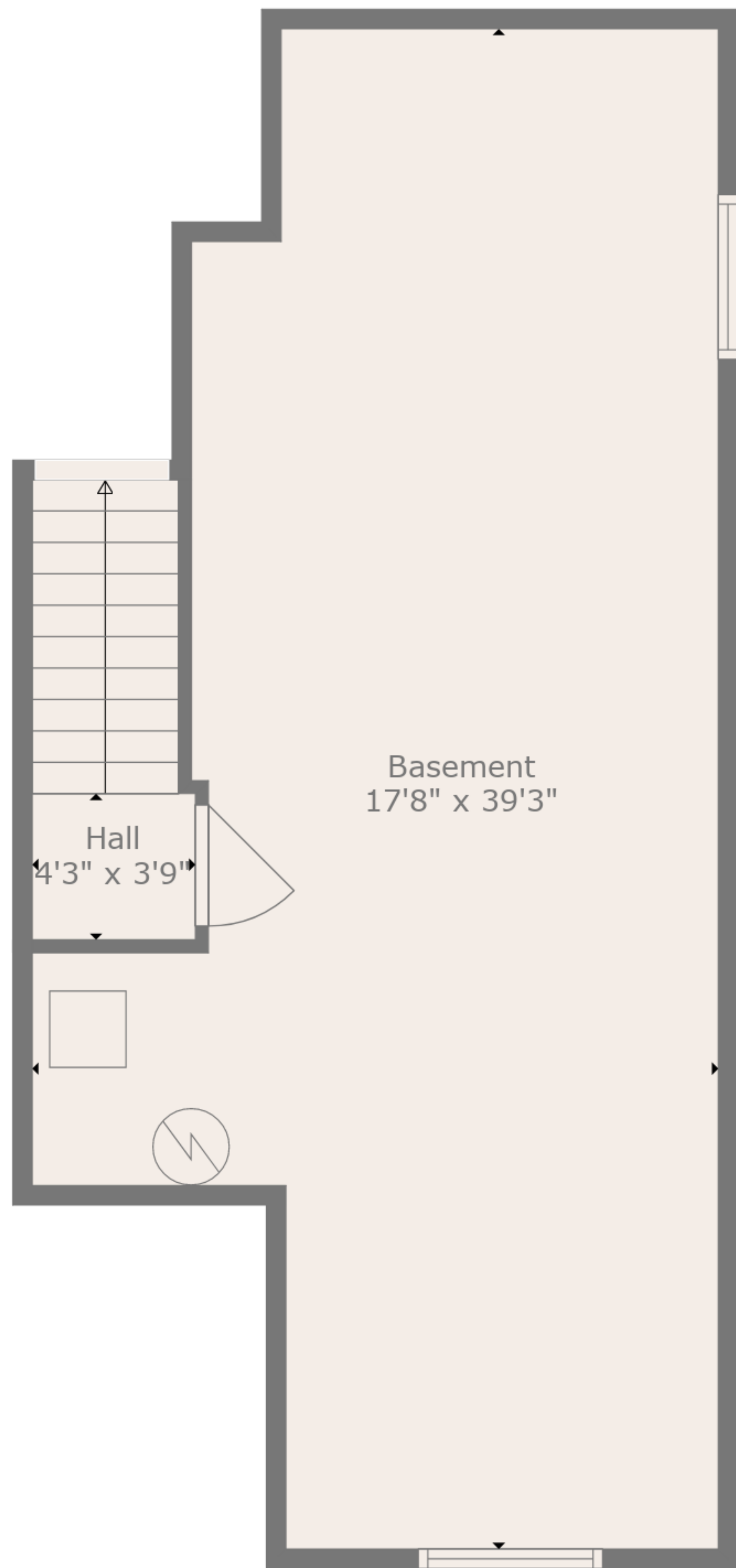
Floor 1
