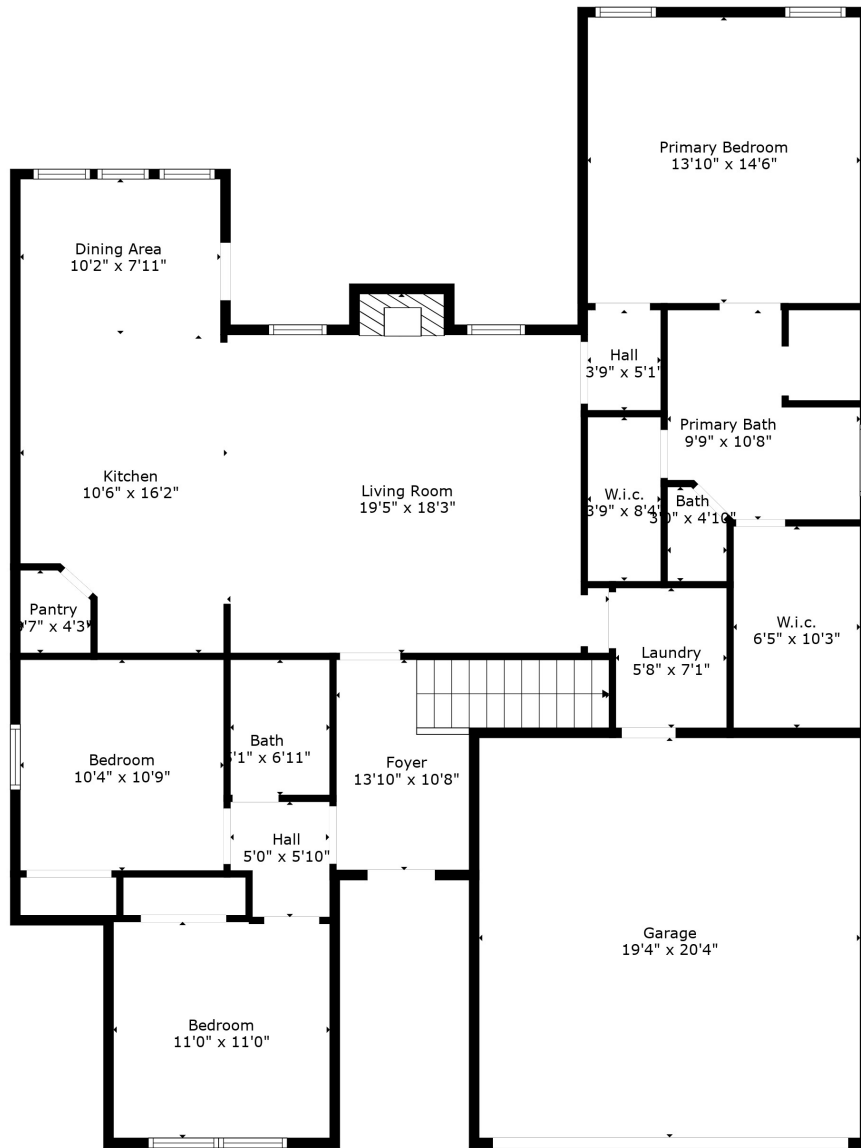
Floor 1
