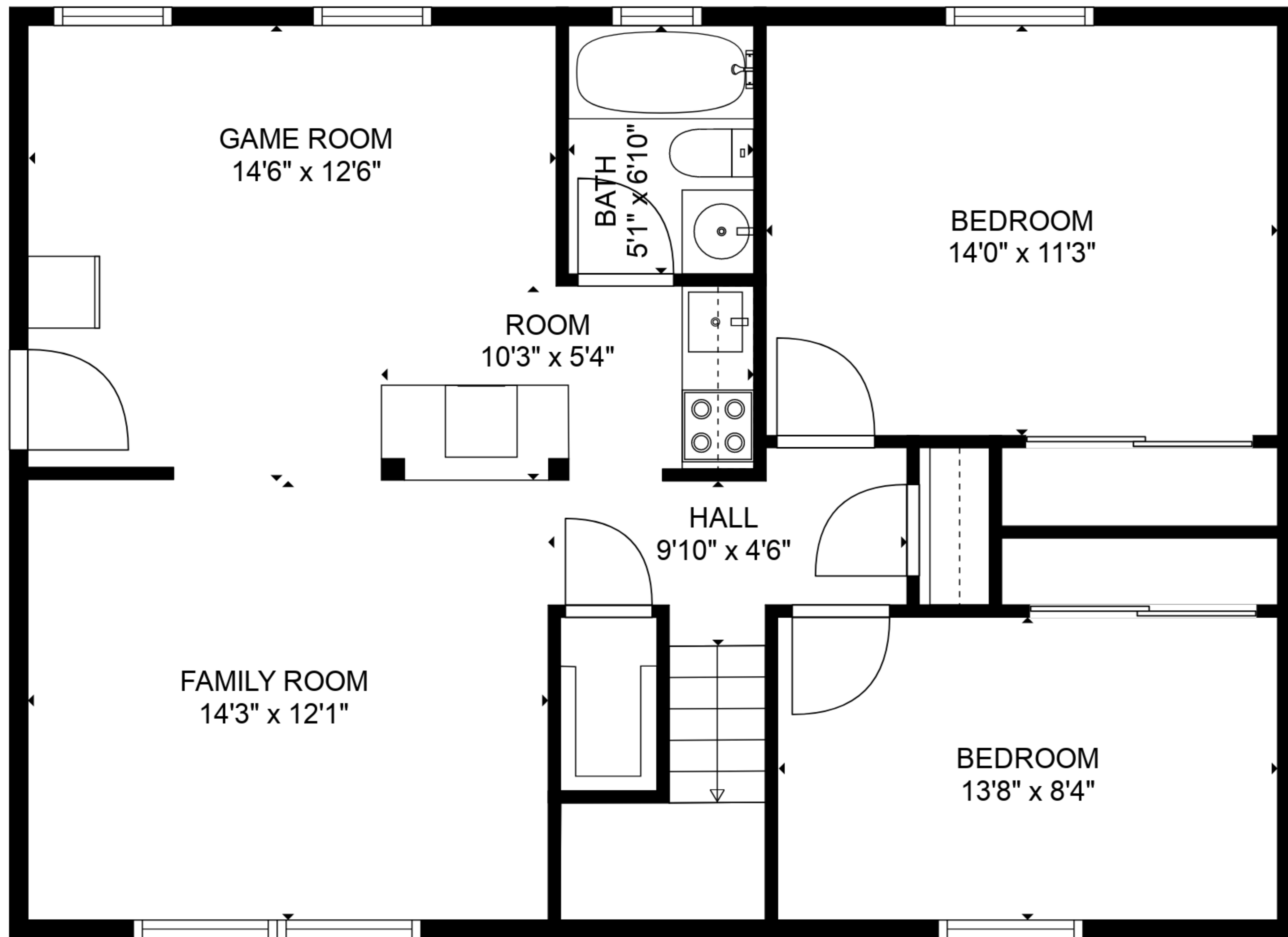
FLOOR 1
