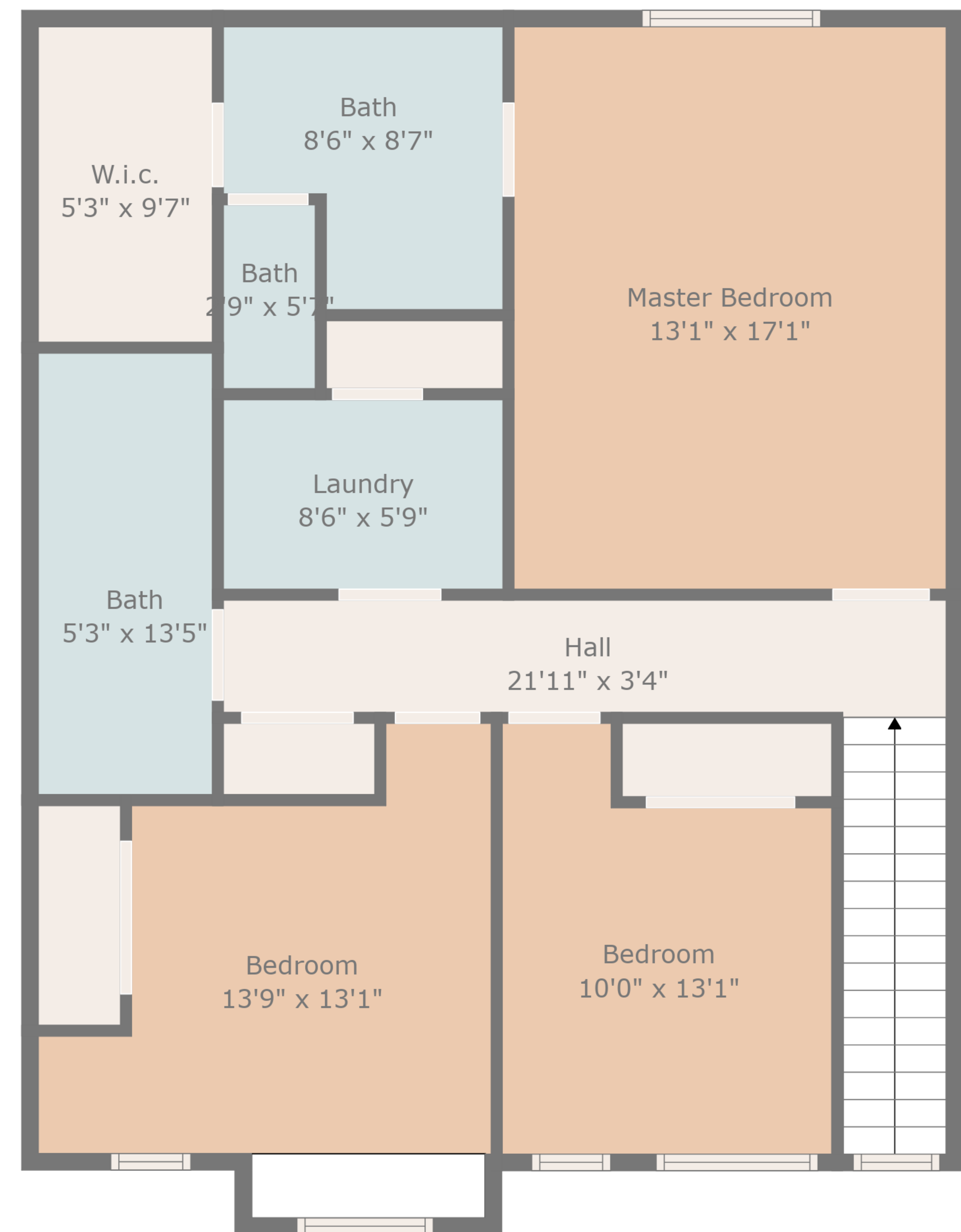
Floor 2
