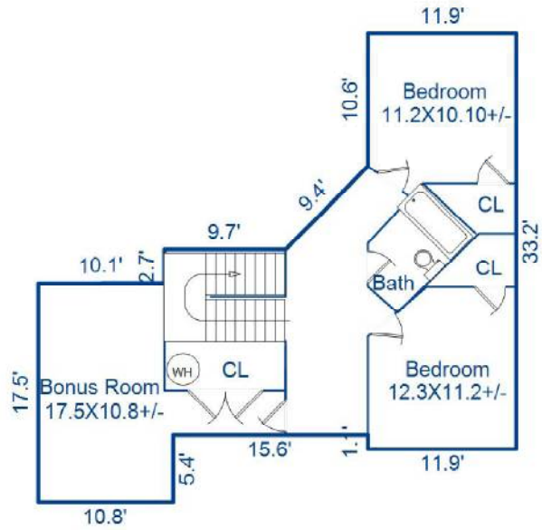
Second Floor 839.2 sf
