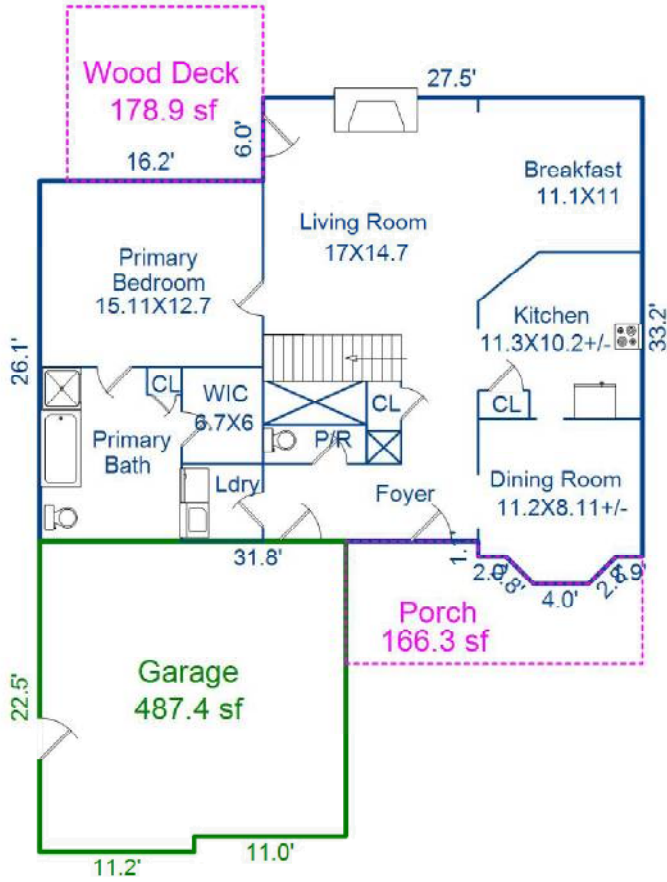
First Floor 1330.7 sf
