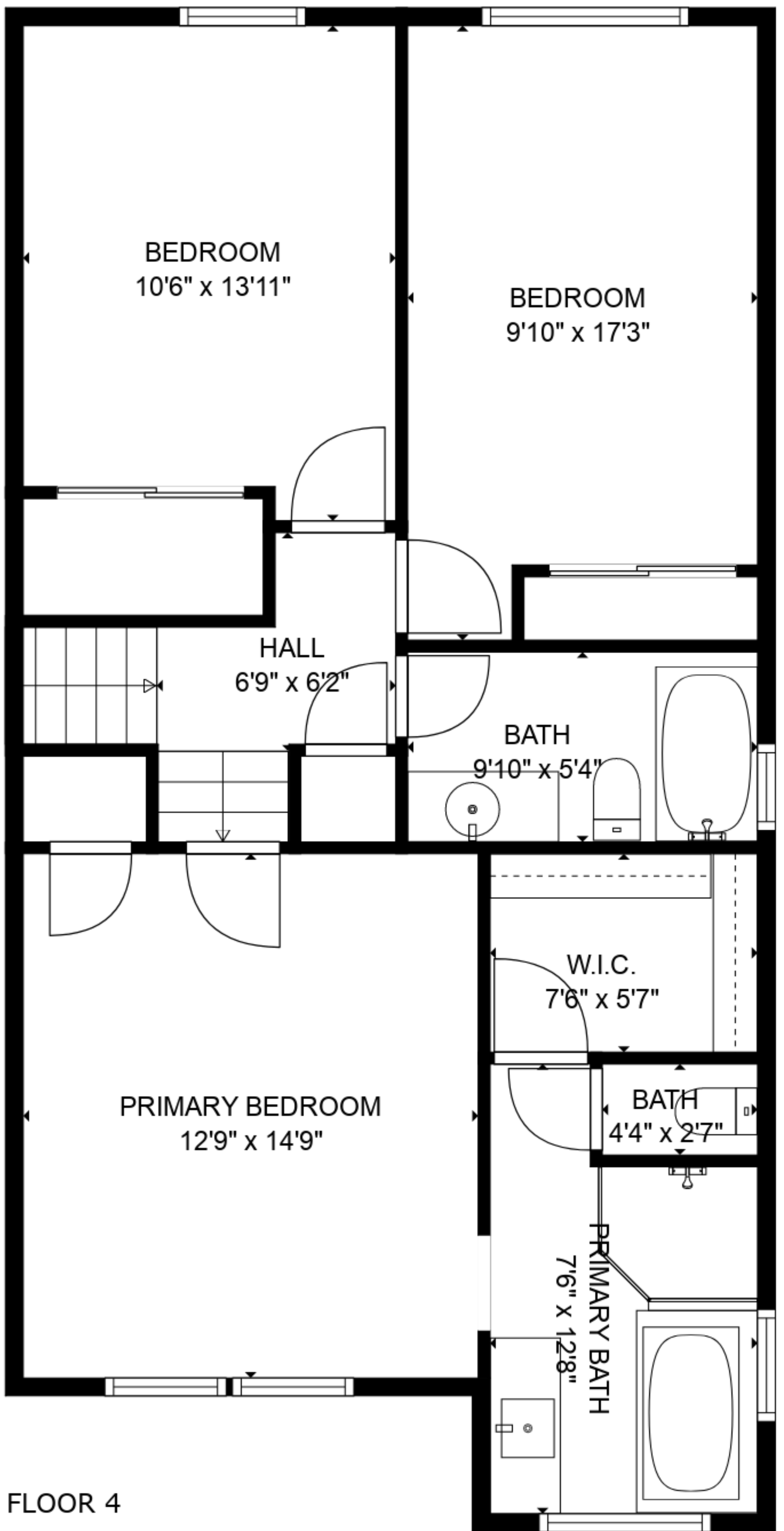
FLOOR 4
