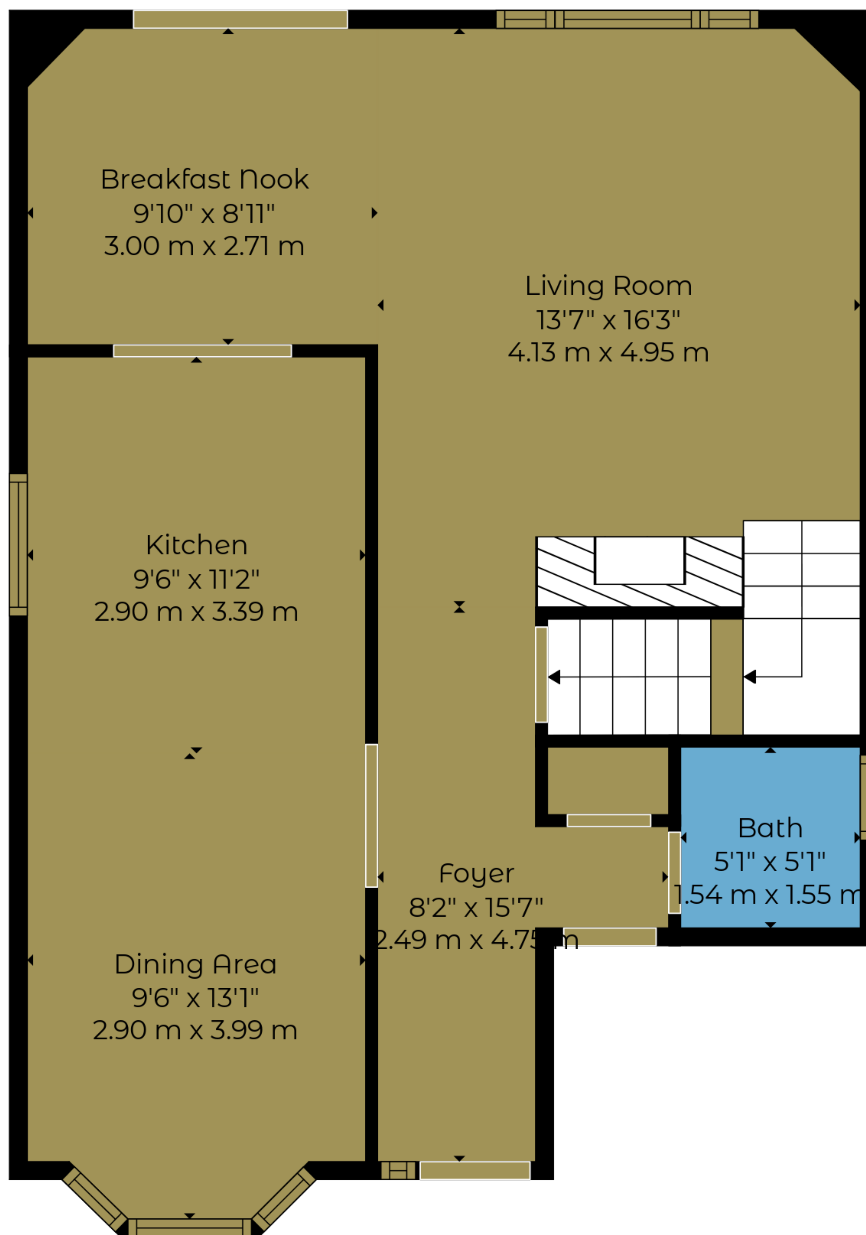
Floor 2
